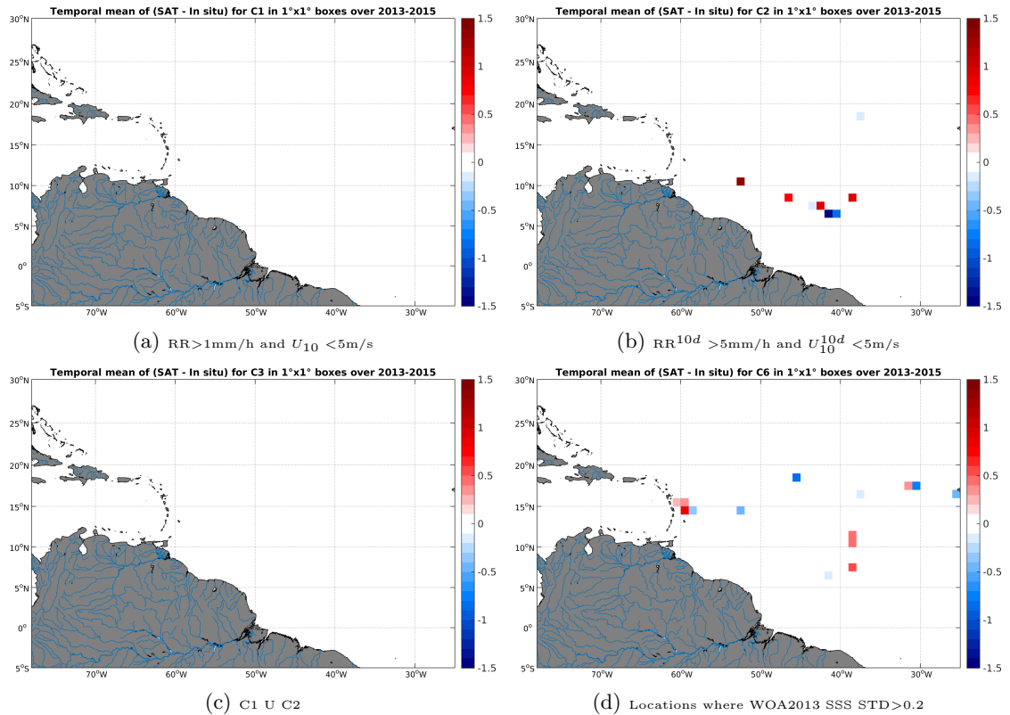
Figure 12: Temporal mean gridded over spatial boxes of size 1^\circ \times 1^\circ of \Delta SSS (SMOS-L2-DPGS-v662 - TSG-GOSUD-Sailing-ship) for 4 different subdatasets corresponding to:RR >1 mm/h and U_{10} < 5 m/s (a), RR^{10d} > 5 mm/h and U_{10}^{10d} < 5 m/s (b), C1 U C2 (c),Locations where WOA2013 SSS STD >0.2 (d).
