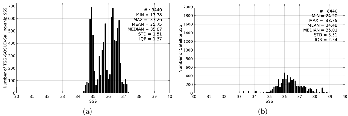
Figure 2: Histograms of SSS from TSG-GOSUD-Sailing-ship (a) and SMOS-L2-DPGS-v662 (b) considering all match-up pairs per bins of 0.1 over the Amazon and Orinoco river plumes Pi-MEP region and for the full satellite product period.
