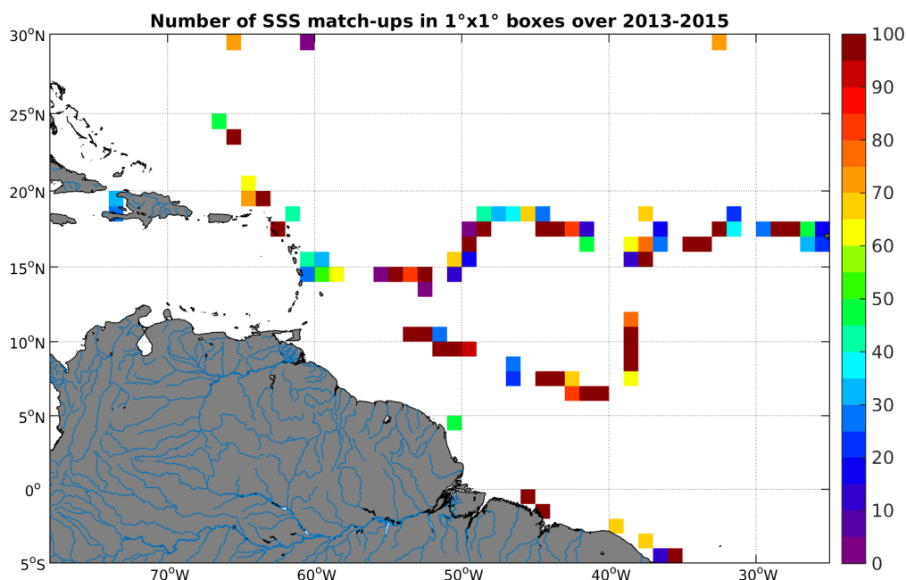
Figure 4: Number of SSS match-ups between TSG-GOSUD-Sailing-ship SSS and the SMOS-L2-DPGS-v662 SSS product for the Amazon and Orinoco river plumes Pi-MEP region over 1°x1° boxes and for the full satellite product period.
