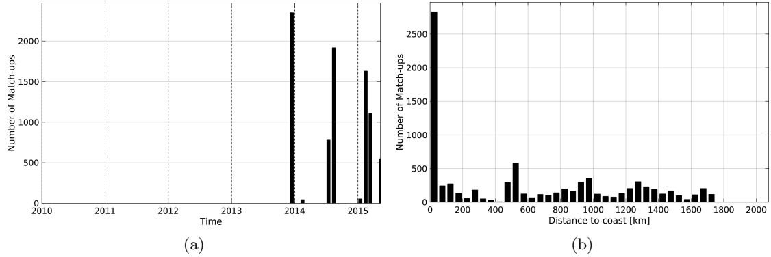
Figure 1: Number of match-ups between TSG-GOSUD-Sailing-ship and SMOS-L2-DPGS-v662 SSS as a function of time (a) and as function of the distance to coast (b) over the Amazon and Orinoco river plumes Pi-MEP region and for the full satellite product period.
