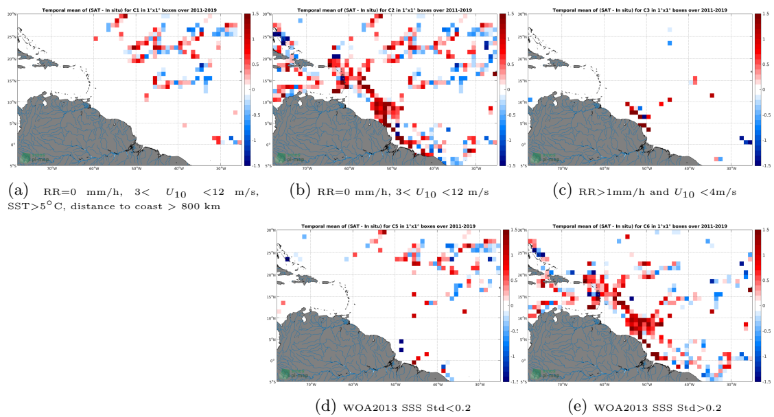
Figure 12: Temporal mean gridded over spatial boxes of size 1^\circ \times 1^\circ of \Delta SSS (SMOS SSS L2 v662 (ESA) - TSG (GOSUD-Research-vessel)) for 5 different subdatasets corresponding to:RR=0 mm/h, 3 < U_{10} < 12 m/s, SST > 5°C, distance to coast > 800 km (a), RR=0 mm/h, 3 < U_{10} < 12 m/s (b), RR > 1mm/h and U_{10} < 4 m/s (c), WOA2013 SSS Std < 0.2 (d), WOA2013 SSS Std > 0.2 (e).
