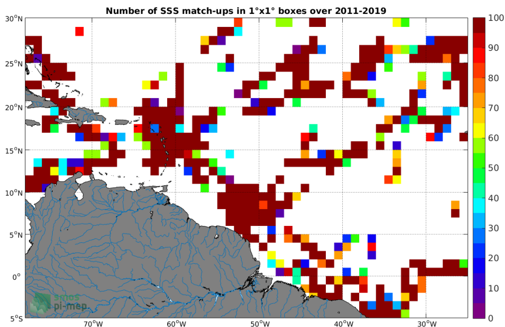
Figure 4: Number of SSS match-ups between TSG (GOSUD-Research-vessel) SSS and the SMOS SSS L2 v662 (ESA) SSS product for the Amazon and Orinoco river plumes Pi-MEP region over 1^{\circ} \times 1^{\circ} boxes and for the full satellite product period.
