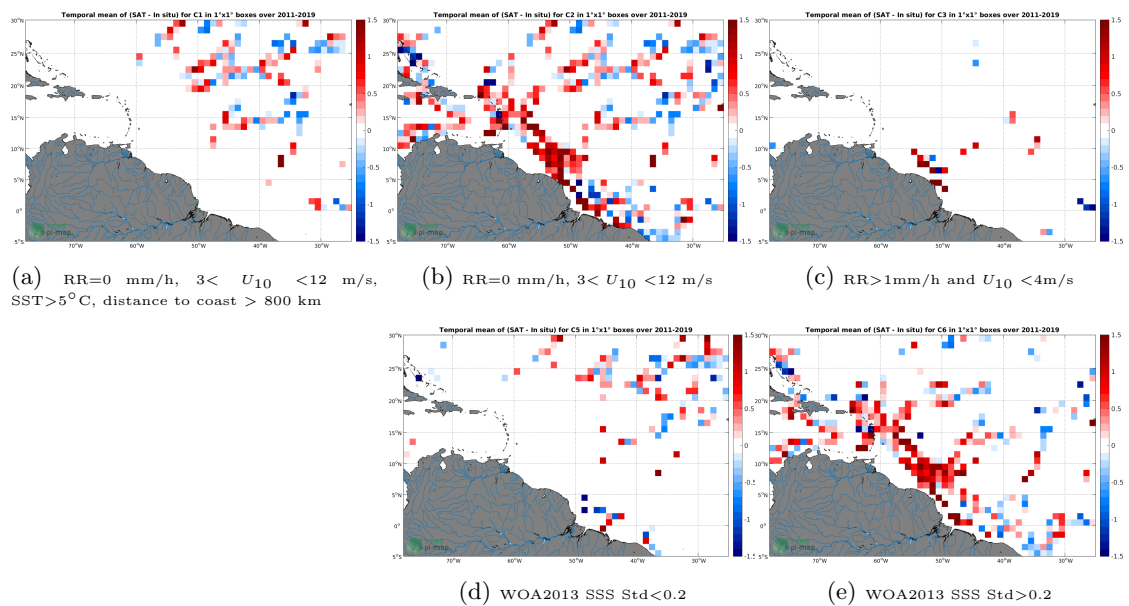
Figure 12: Temporal mean gridded over spatial boxes of size 1°x1° of \Delta SSS (SMOS SSS L2 v662 (ESA) - TSG (GOSUD-Research-vessel)) for 5 different subdatasets corresponding to: RR=0 mm/h, 3 < U_{10} < 12 m/s, SST > 5°C, distance to coast > 800 km (a), RR=0 mm/h, 3 < U_{10} < 12 m/s (b), RR > 1mm/h and U_{10} < 4 m/s (c), WOA2013 SSS Std < 0.2 (d), WOA2013 SSS Std > 0.2 (e).
