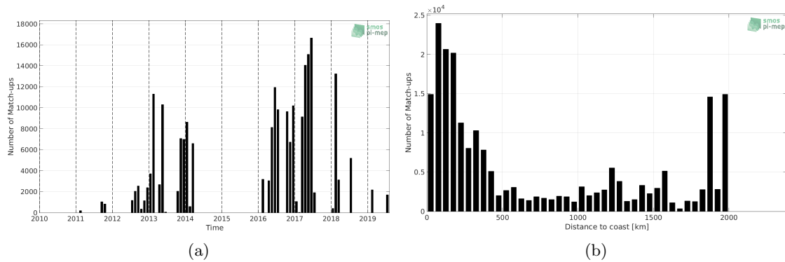
Figure 1: Number of match-ups between TSG (GOSUD-Research-vessel) and SMOS SSS L2 v662 (ESA) SSS as a function of time (a) and as function of the distance to coast (b) over the Amazon and Orinoco river plumes Pi-MEP region and for the full satellite product period.
