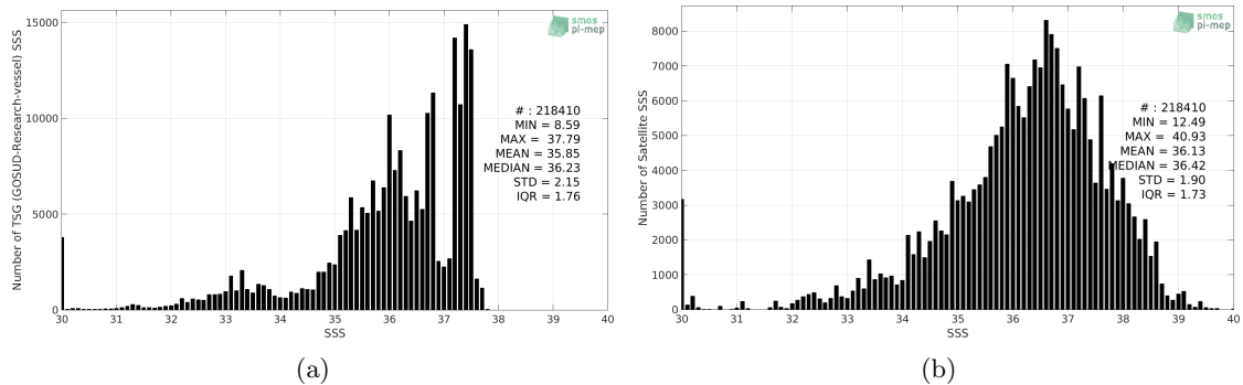
Figure 2: Histograms of SSS from TSG (GOSUD-Research-vessel) (a) and SMOS SSS L2 v662 (ESA) (b) considering all match-up pairs per bins of 0.1 over the Amazon and Orinoco river plumes Pi-MEP region and for the full satellite product period.
