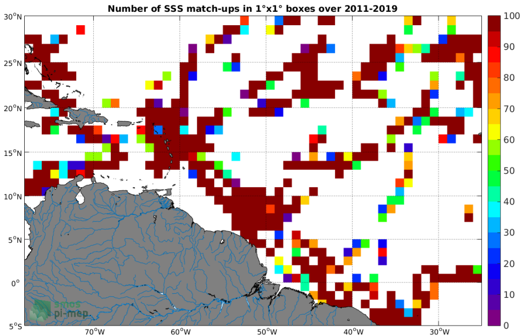
Figure 4: Number of SSS match-ups between TSG (GOSUD-Research-vessel) SSS and the SMOS SSS L2 v662 (ESA) SSS product for the Amazon and Orinoco river plumes Pi-MEP region over 1°x1° boxes and for the full satellite product period.
