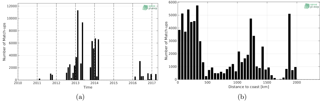
Figure 1: Number of match-ups between TSG-GOSUD-Research-vessel and SMOS-L2-DPGS-v662 SSS as a function of time (a) and as function of the distance to coast (b) over the Amazon and Orinoco river plumes Pi-MEP region and for the full satellite product period.
