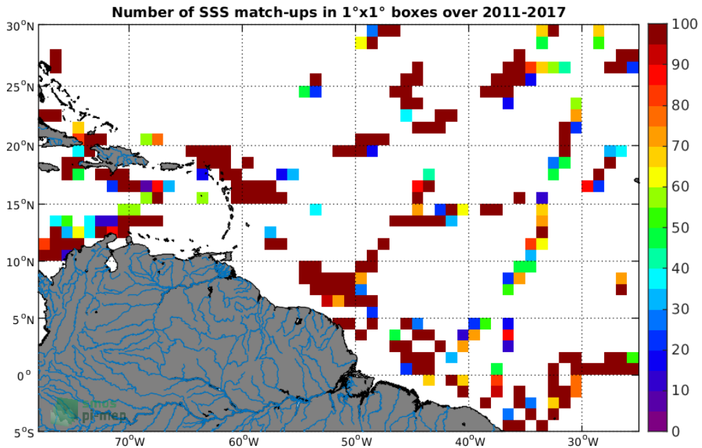
Figure 4: Number of SSS match-ups between TSG-GOSUD-Research-vessel SSS and the SMOS-L2-DPGS-v662 SSS product for the Amazon and Orinoco river plumes Pi-MEP region over 1°x1° boxes and for the full satellite product period.
