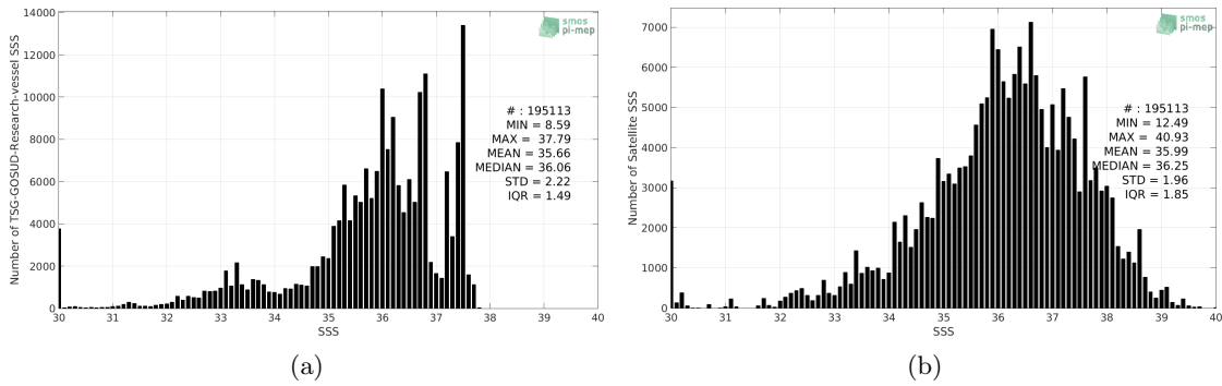
Figure 2: Histograms of SSS from TSG-GOSUD-Research-vessel (a) and SMOS-L2-DPGS-v662 (b) considering all match-up pairs per bins of 0.1 over the Amazon and Orinoco river plumes Pi-MEP region and for the full satellite product period.
