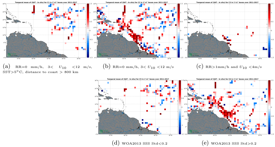
Figure 12: Temporal mean gridded over spatial boxes of size 1^\circ \times 1^\circ of \Delta SSS (SMOS-L2-DPGS-v662 - TSG-GOSUD-Research-vessel) for 5 different subdatasets corresponding to:RR=0 mm/h, 3 < U_{10} < 12 m/s, SST >5^\circ\text{C} , distance to coast > 800 km (a), RR=0 mm/h, 3 < U_{10} < 12 m/s (b), RR >1 mm/h and U_{10} < 4 m/s (c), WOA2013 SSS Std <0.2 (d), WOA2013 SSS Std >0.2 (e).
