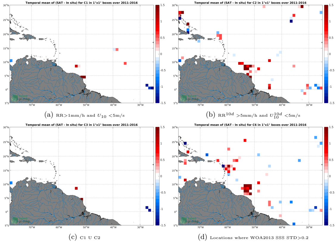
Figure 12: Temporal mean gridded over spatial boxes of size 1^\circ \times 1^\circ of \Delta SSS (SMOS-L2-DPGS-v662 - TSG-GOSUD-Research-vessel) for 4 different subdatasets corresponding to: RR > 1\text{mm/h} and U_{10} < 5\text{m/s} (a), RR^{10d} > 5\text{mm/h} and U_{10}^{10d} < 5\text{m/s} (b), C1 U C2 (c), Locations where WOA2013 SSS STD > 0.2 (d).
