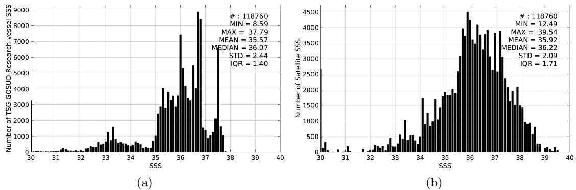
Figure 2: Histograms of SSS from TSG-GOSUD-Research-vessel (a) and SMOS-L2-DPGS-v662 (b) considering all match-up pairs per bins of 0.1 over the Amazon and Orinoco river plumes Pi-MEP region and for the full satellite product period.
