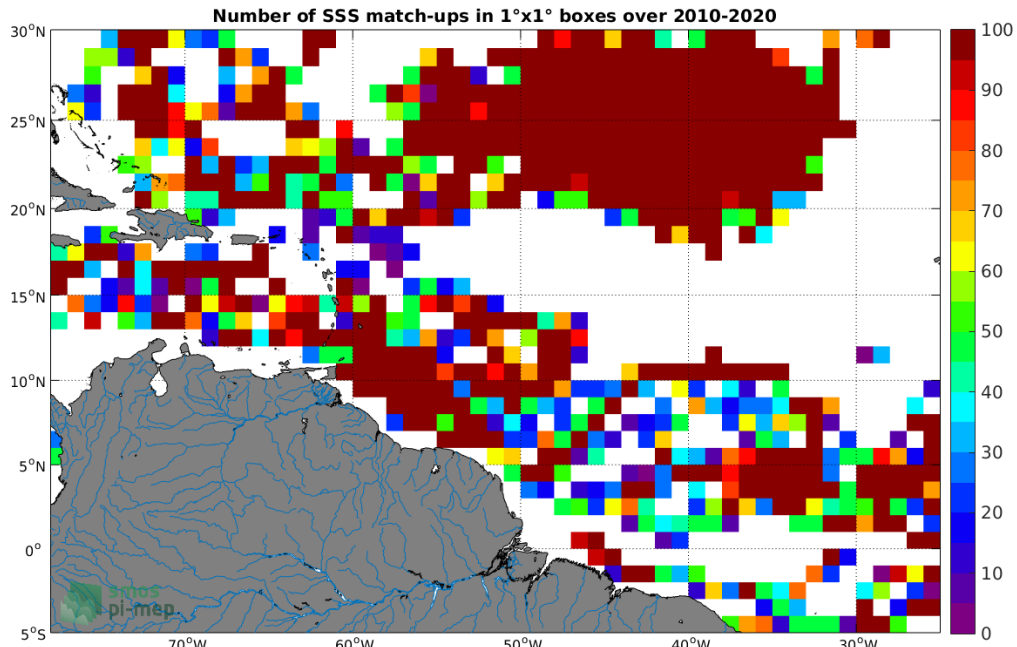
Figure 3: Number of SSS match-ups between Surface drifters SSS and the SMOS SSS L2 v662 (ESA) SSS product for the Amazon and Orinoco river plumes Pi-MEP region over 1^\circ \times 1^\circ boxes and for the full satellite product period.
