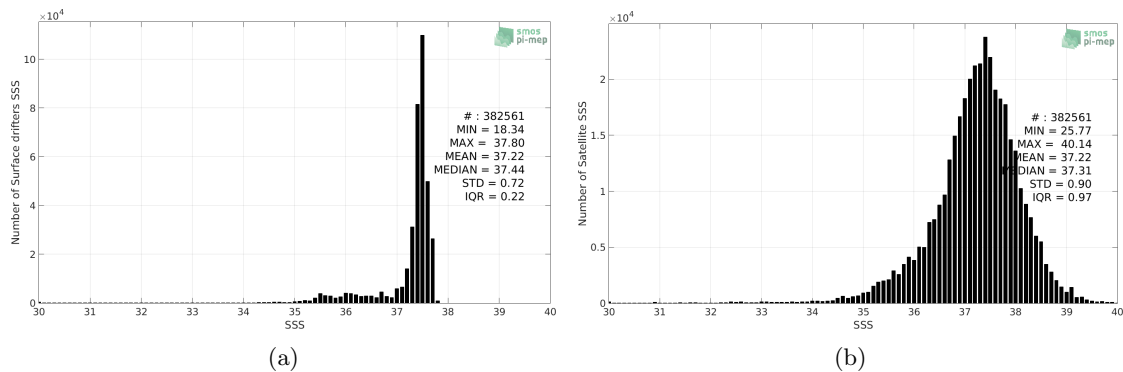
Figure 2: Histograms of SSS from Surface drifters (a) and SMOS SSS L2 v662 (ESA) (b) considering all match-up pairs per bins of 0.1 over the Amazon and Orinoco river plumes Pi-MEP region and for the full satellite product period.
