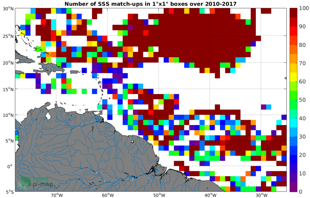
Figure 3: Number of SSS match-ups between Surface drifters SSS and the SMOS SSS L2 v662 (ESA) SSS product for the Amazon and Orinoco river plumes Pi-MEP region over 1°x1° boxes and for the full satellite product period.
