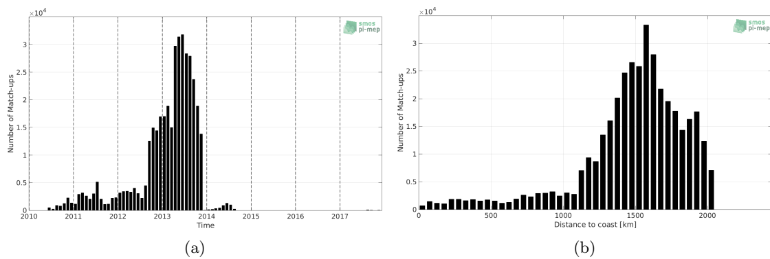
Figure 1: Number of match-ups between Surface drifters and SMOS SSS L2 v662 (ESA) SSS as a function of time (a) and as function of the distance to coast (b) over the Amazon and Orinoco river plumes Pi-MEP region and for the full satellite product period.
