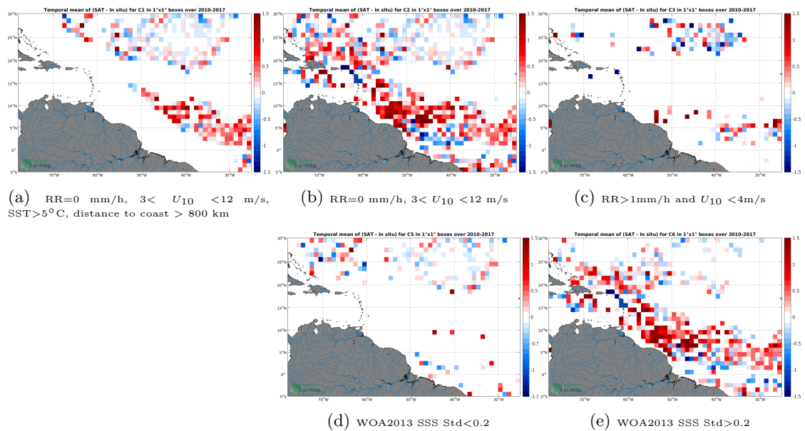
Figure 11: Temporal mean gridded over spatial boxes of size 1°x1° of \Delta SSS (SMOS SSS L2 v662 (ESA) - Surface drifters) for 5 different subdatasets corresponding to: RR=0 mm/h, 3 < U_{10} < 12 m/s, SST > 5°C, distance to coast > 800 km (a), RR=0 mm/h, 3 < U_{10} < 12 m/s (b), RR > 1mm/h and U_{10} < 4 m/s (c), WOA2013 SSS Std < 0.2 (d), WOA2013 SSS Std > 0.2 (e).
