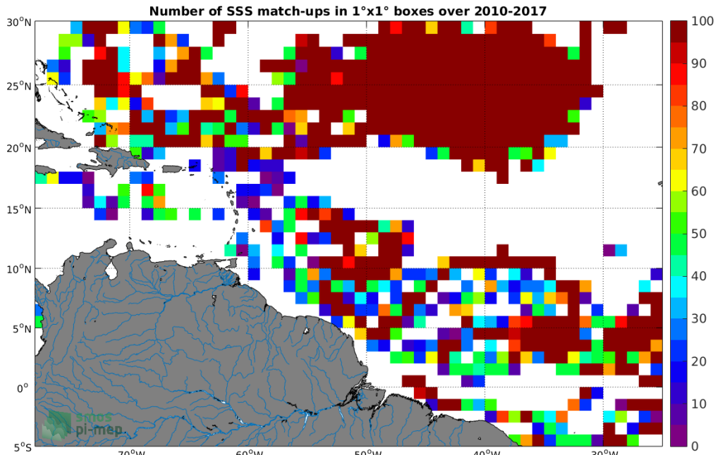
Figure 3: Number of SSS match-ups between Surface drifters SSS and the SMOS L2 v662 (ESA) SSS product for the Amazon and Orinoco river plumes Pi-MEP region over 1^\circ \times 1^\circ boxes and for the full satellite product period.
