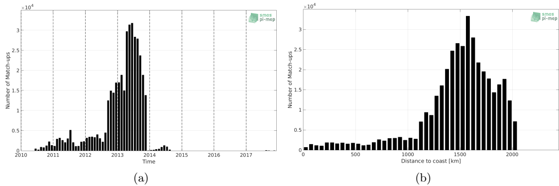
Figure 1: Number of match-ups between Surface drifters and SMOS L2 v662 (ESA) SSS as a function of time (a) and as function of the distance to coast (b) over the Amazon and Orinoco river plumes Pi-MEP region and for the full satellite product period.
