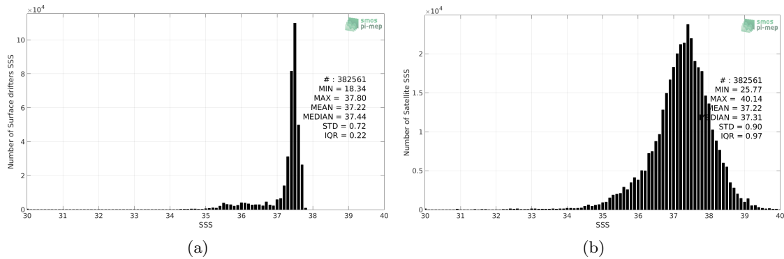
Figure 2: Histograms of SSS from Surface drifters (a) and SMOS L2 v662 (ESA) (b) considering all match-up pairs per bins of 0.1 over the Amazon and Orinoco river plumes Pi-MEP region and for the full satellite product period.
