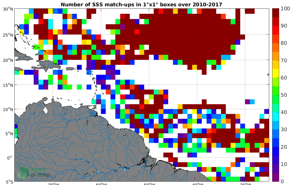
Figure 3: Number of SSS match-ups between Surface drifters SSS and the SMOS-L2-DPGS-v662 SSS product for the Amazon and Orinoco river plumes Pi-MEP region over 1^\circ \times 1^\circ boxes and for the full satellite product period.
