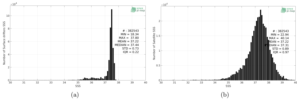
Figure 2: Histograms of SSS from Surface drifters (a) and SMOS-L2-DPGS-v662 (b) considering all match-up pairs per bins of 0.1 over the Amazon and Orinoco river plumes Pi-MEP region and for the full satellite product period.
