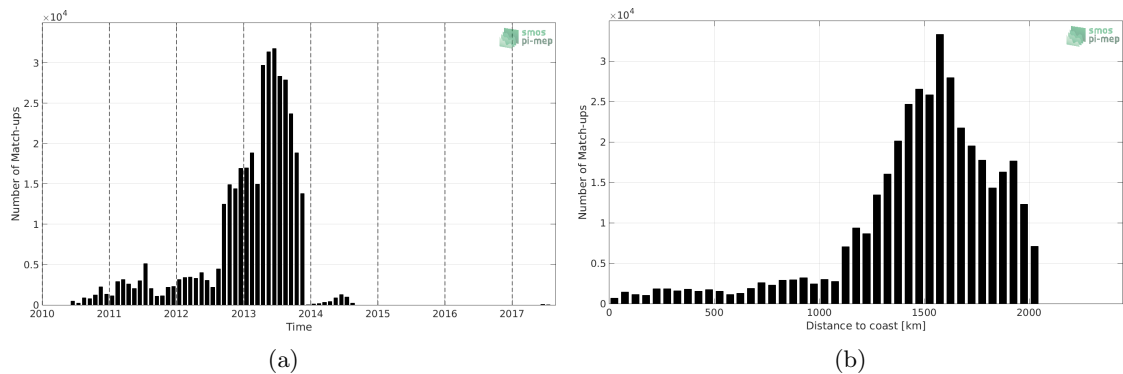
Figure 1: Number of match-ups between Surface drifters and SMOS-L2-DPGS-v662 SSS as a function of time (a) and as function of the distance to coast (b) over the Amazon and Orinoco river plumes Pi-MEP region and for the full satellite product period.
