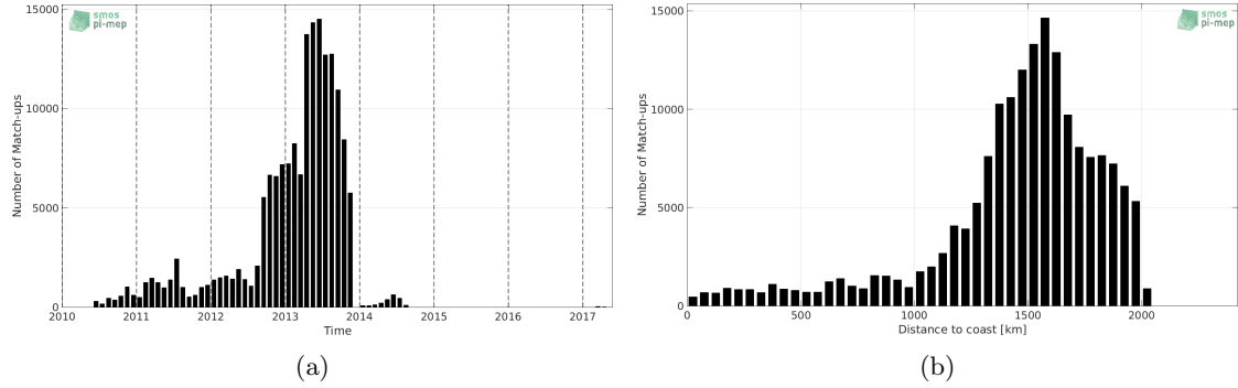
Figure 1: Number of match-ups between Surface drifters and SMOS-L2-DPGS-v662 SSS as a function of time (a) and as function of the distance to coast (b) over the Amazon and Orinoco river plumes Pi-MEP region and for the full satellite product period.
