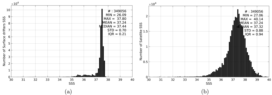
Figure 2: Histograms of SSS from Surface drifters (a) and SMOS-L2-DPGS-v662 (b) considering all match-up pairs per bins of 0.1 over the Amazon and Orinoco river plumes Pi-MEP region and for the full satellite product period.
