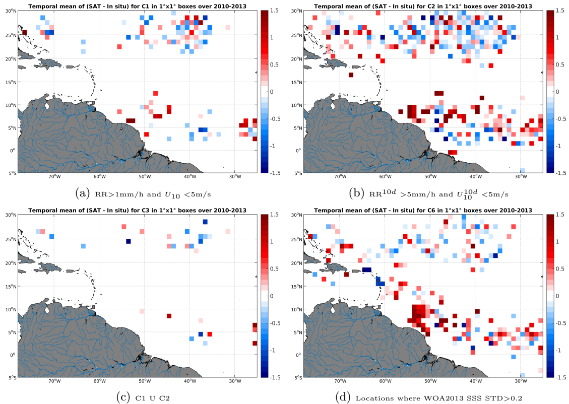
Figure 11: Temporal mean gridded over spatial boxes of size 1^\circ \times 1^\circ of \Delta SSS (SMOS-L2-DPGS-v662 - Surface drifters) for 4 different subdatasets corresponding to:RR > 1mm/h and U_{10} < 5 m/s (a), RR^{10d} > 5 mm/h and U_{10}^{10d} < 5 m/s (b), C1 U C2 (c),Locations where WOA2013 SSS STD > 0.2 (d).
