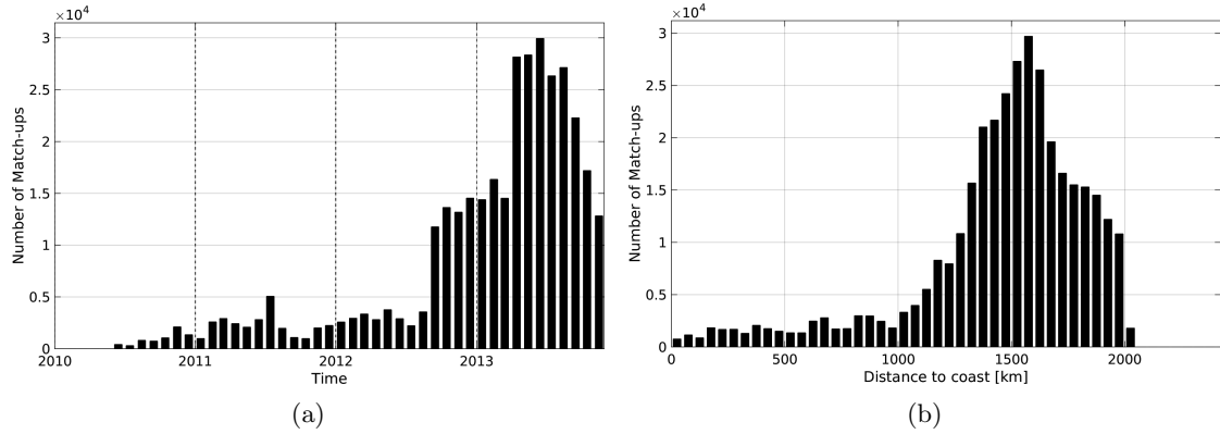
Figure 1: Number of match-ups between Surface drifters and SMOS-L2-DPGS-v662 SSS as a function of time (a) and as function of the distance to coast (b) over the Amazon and Orinoco river plumes Pi-MEP region and for the full satellite product period.
