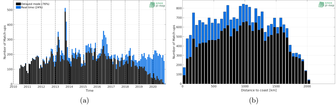
Figure 1: Number of match-ups between Argo and SMOS SSS L2 v662 (ESA) SSS as a function of time (a) and as function of the distance to coast (b) over the Amazon and Orinoco river plumes Pi-MEP region and for the full satellite product period.
