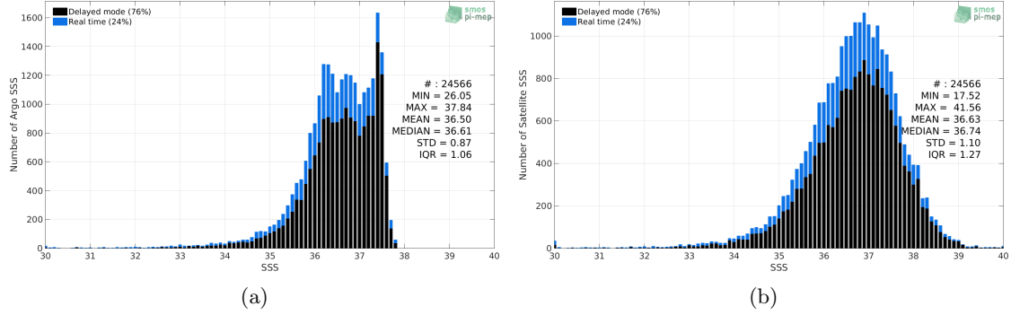
Figure 2: Histograms of SSS from Argo (a) and SMOS SSS L2 v662 (ESA) (b) considering all match-up pairs per bins of 0.1 over the Amazon and Orinoco river plumes Pi-MEP region and for the full satellite product period.
