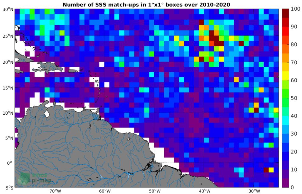
Figure 4: Number of SSS match-ups between Argo SSS and the SMOS SSS L2 v662 (ESA) SSS product for the Amazon and Orinoco river plumes Pi-MEP region over 1^\circ \times 1^\circ boxes and for the full satellite product period.
