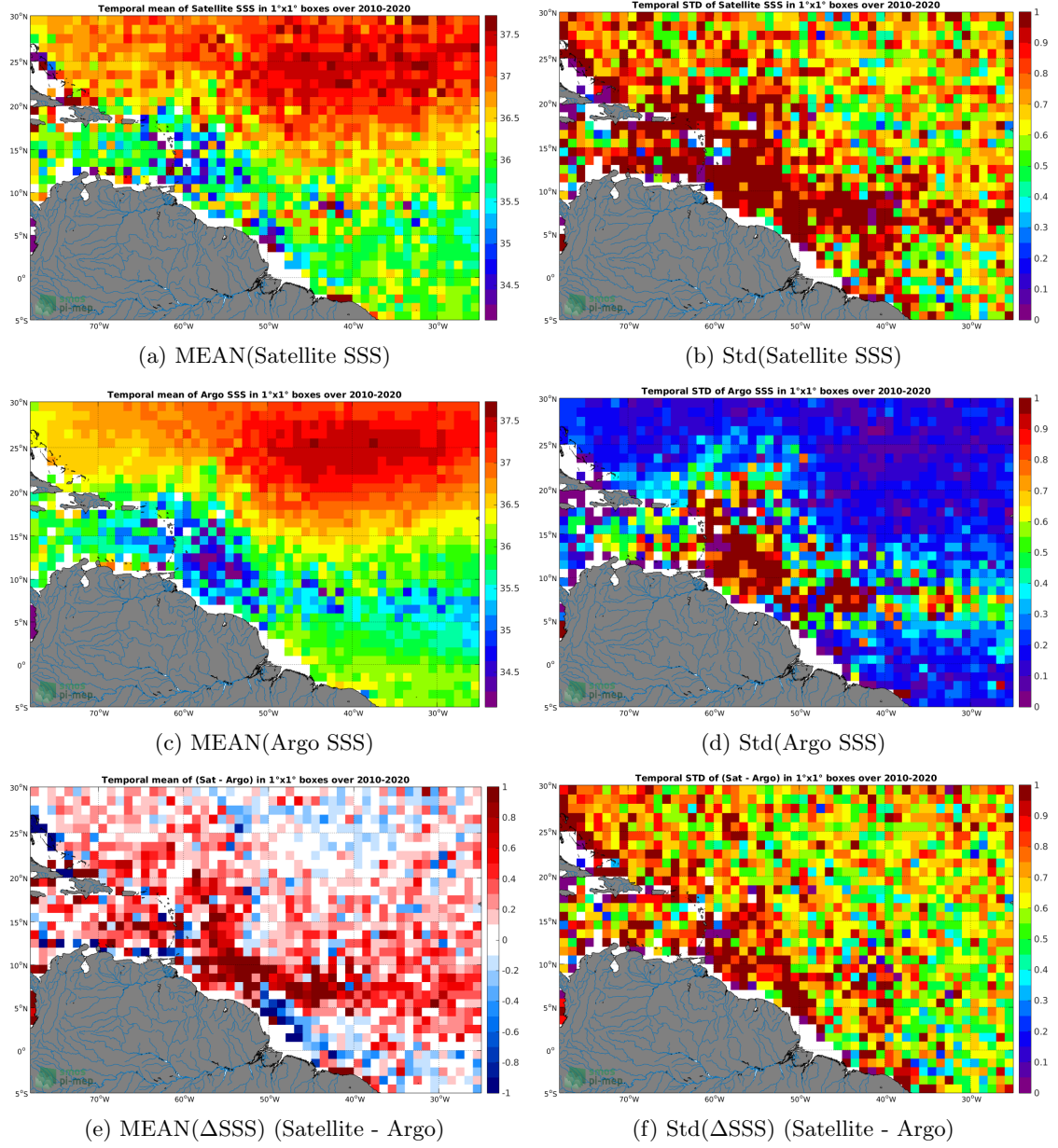
Figure 6: Temporal mean (left) and Std (right) of SSS from SMOS L2 v662 (ESA) (top), Argo (middle), and of \Delta SSS (Satellite - Argo). Only match-up pairs are used to generate these maps.
