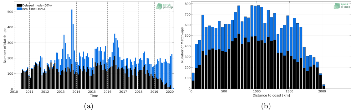
Figure 1: Number of match-ups between Argo and SMOS L2 v662 (ESA) SSS as a function of time (a) and as function of the distance to coast (b) over the Amazon and Orinoco river plumes Pi-MEP region and for the full satellite product period.
