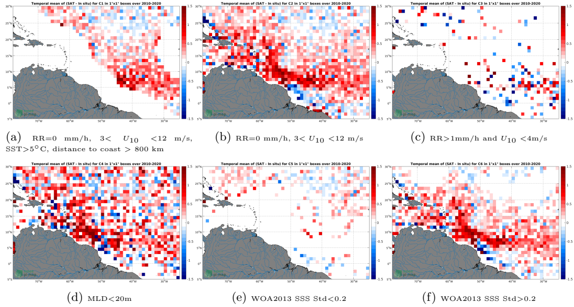
Figure 12: Temporal mean gridded over spatial boxes of size 1^\circ \times 1^\circ of \Delta SSS (SMOS L2 v662 (ESA) - Argo) for 6 different subdatasets corresponding to: RR=0 mm/h, 3 < U_{10} < 12 m/s, SST > 5^\circ C , distance to coast > 800 km (a), RR=0 mm/h, 3 < U_{10} < 12 m/s (b), RR > 1 mm/h and U_{10} < 4 m/s (c), MLD < 20 m (d), WOA2013 SSS Std < 0.2 (e), WOA2013 SSS Std > 0.2 (f).
