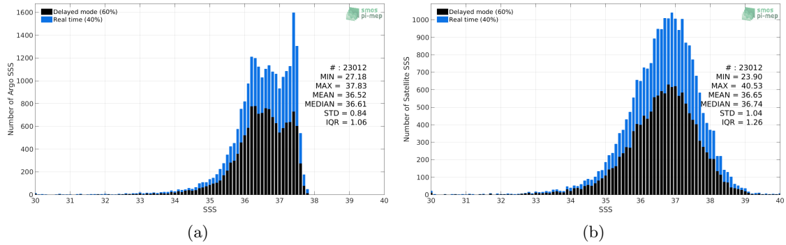
Figure 2: Histograms of SSS from Argo (a) and SMOS L2 v662 (ESA) (b) considering all match-up pairs per bins of 0.1 over the Amazon and Orinoco river plumes Pi-MEP region and for the full satellite product period.
