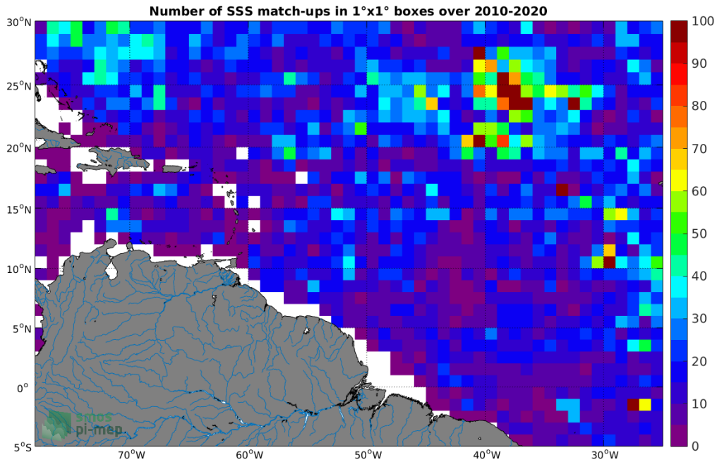
Figure 4: Number of SSS match-ups between Argo SSS and the SMOS L2 v662 (ESA) SSS product for the Amazon and Orinoco river plumes Pi-MEP region over 1°x1° boxes and for the full satellite product period.
