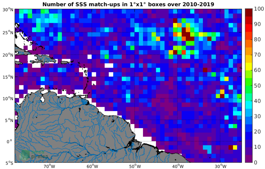
Figure 4: Number of SSS match-ups between Argos SSS and the SMOS-L2-DPGS-v662 SSS product for the Amazon and Orinoco river plumes Pi-MEP region over 1°x1° boxes and for the full satellite product period.
