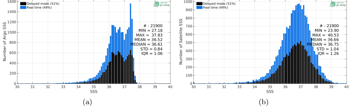
Figure 2: Histograms of SSS from Argo (a) and SMOS-L2-DPGS-v662 (b) considering all match-up pairs per bins of 0.1 over the Amazon and Orinoco river plumes Pi-MEP region and for the full satellite product period.
