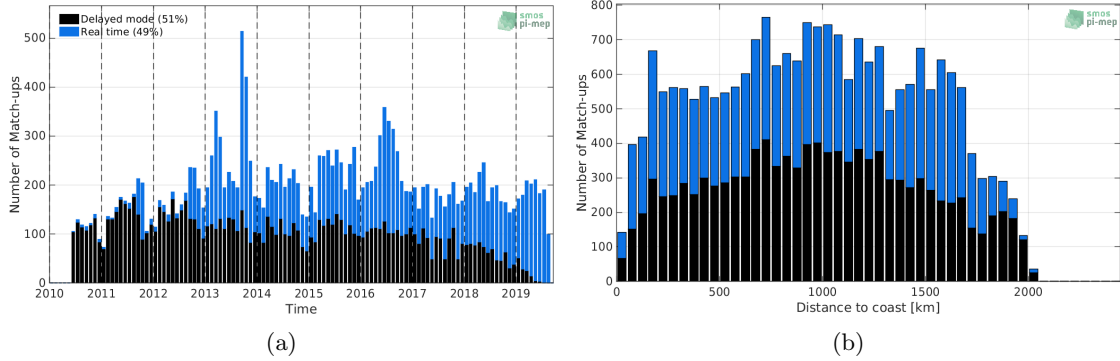
Figure 1: Number of match-ups between Argo and SMOS-L2-DPGS-v662 SSS as a function of time (a) and as function of the distance to coast (b) over the Amazon and Orinoco river plumes Pi-MEP region and for the full satellite product period.
