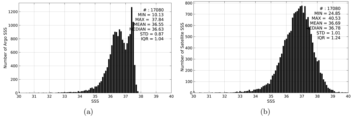
Figure 2: Histograms of SSS from Argo (a) and SMOS-L2-DPGS-v662 (b) considering all match-up pairs per bins of 0.1 over the Amazon and Orinoco river plumes Pi-MEP region and for the full satellite product period.
