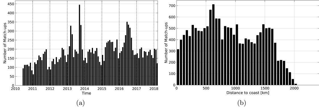
Figure 1: Number of match-ups between Argo and SMOS-L2-DPGS-v662 SSS as a function of time (a) and as function of the distance to coast (b) over the Amazon and Orinoco river plumes Pi-MEP region and for the full satellite product period.
