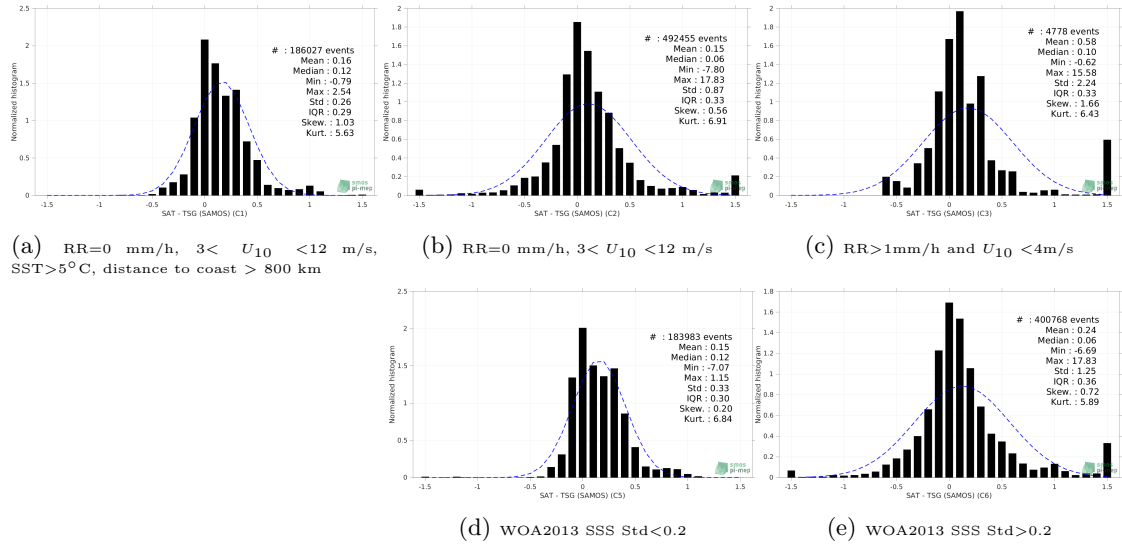
Figure 13: Normalized histogram of \Delta\text{SSS} (SMAP SSS L4 OI v1 - 7 Days (IPRC) - TSG (SAMOS)) for 5 different subdatasets corresponding to: RR=0 mm/h, 3 < U_{10} < 12 m/s, SST>5°C, distance to coast > 800 km (a), RR=0 mm/h, 3 < U_{10} < 12 m/s (b), RR>1mm/h and U_{10} < 4 m/s (c), WOA2013 SSS Std<0.2 (d), WOA2013 SSS Std>0.2 (e).
