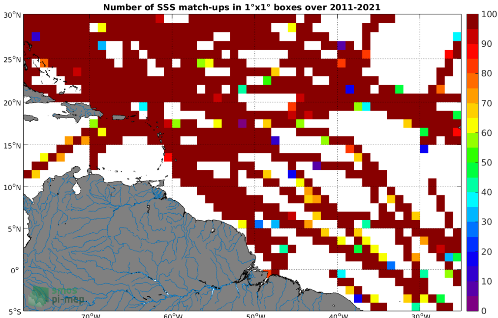
Figure 4: Number of SSS match-ups between TSG (SAMOS) SSS and the SMAP SSS L4 OI v1 - 7day (IPRC) SSS product for the Amazon and Orinoco river plumes Pi-MEP region over 1^{\circ} \times 1^{\circ} boxes and for the full satellite product period.
