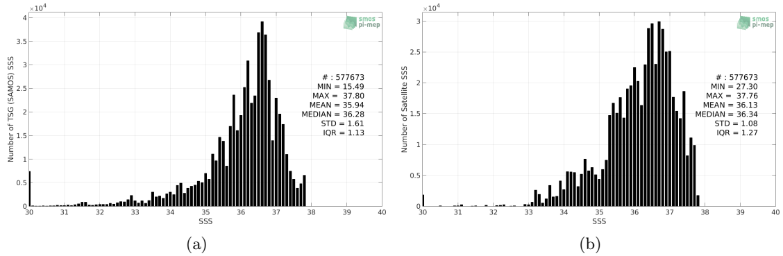
Figure 2: Histograms of SSS from TSG (SAMOS) (a) and SMAP SSS L4 OI v1 - 7day (IPRC) (b) considering all match-up pairs per bins of 0.1 over the Amazon and Orinoco river plumes Pi-MEP region and for the full satellite product period.
