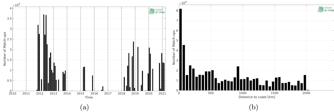
Figure 1: Number of match-ups between TSG (SAMOS) and SMAP SSS L4 OI v1 - 7day (IPRC) SSS as a function of time (a) and as function of the distance to coast (b) over the Amazon and Orinoco river plumes Pi-MEP region and for the full satellite product period.
