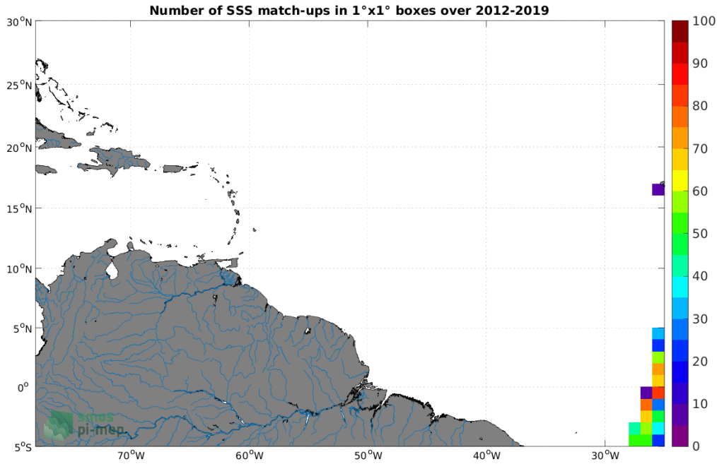
Figure 4: Number of SSS match-ups between TSG (Polarstern) SSS and the SMAP SSS L4 OI v1 - 7 Days (IPRC) SSS product for the Amazon and Orinoco river plumes Pi-MEP region over 1°x1° boxes and for the full satellite product period.
