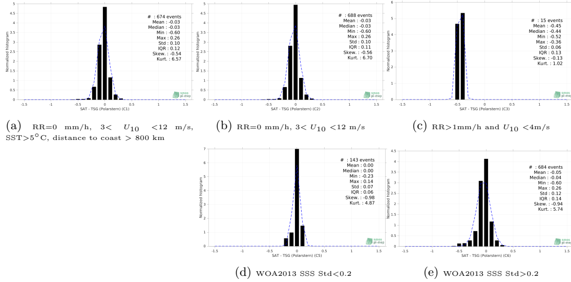
Figure 13: Normalized histogram of \Delta\text{SSS} (SMAP SSS L4 OI v1 - 7 Days (IPRC) - TSG (Polarstern)) for 5 different subdatasets corresponding to: RR=0 mm/h, 3 < U_{10} < 12 m/s, SST>5°C, distance to coast > 800 km (a), RR=0 mm/h, 3 < U_{10} < 12 m/s (b), RR>1mm/h and U_{10} < 4 m/s (c), WOA2013 SSS Std<0.2 (d), WOA2013 SSS Std>0.2 (e).
