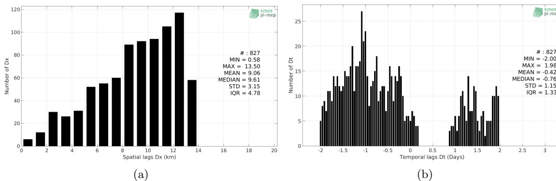
Figure 5: Histograms of the spatial (a) and temporal (b) lags between the location/time of the TSG (Polarstern) measurement and the date of the corresponding SMAP SSS L4 OI v1 - 7 Days (IPRC) SSS pixel.
