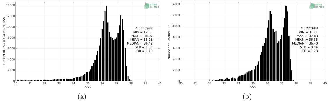
Figure 2: Histograms of SSS from TSG (LEGOS-DM) (a) and SMAP SSS L4 OI v1 - 7day (IPRC) (b) considering all match-up pairs per bins of 0.1 over the Amazon and Orinoco river plumes Pi-MEP region and for the full satellite product period.
