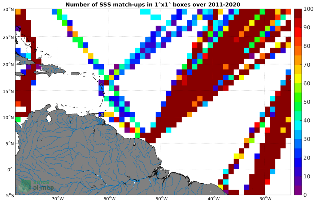
Figure 4: Number of SSS match-ups between TSG (LEGOS-DM) SSS and the SMAP SSS L4 OI v1 - 7day (IPRC) SSS product for the Amazon and Orinoco river plumes Pi-MEP region over 1°x1° boxes and for the full satellite product period.
