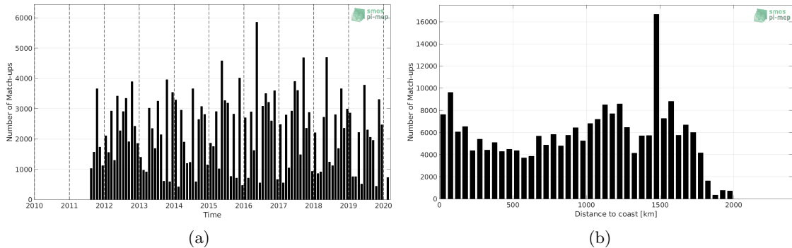
Figure 1: Number of match-ups between TSG (LEGOS-DM) and SMAP SSS L4 OI v1 - 7day (IPRC) SSS as a function of time (a) and as function of the distance to coast (b) over the Amazon and Orinoco river plumes Pi-MEP region and for the full satellite product period.
