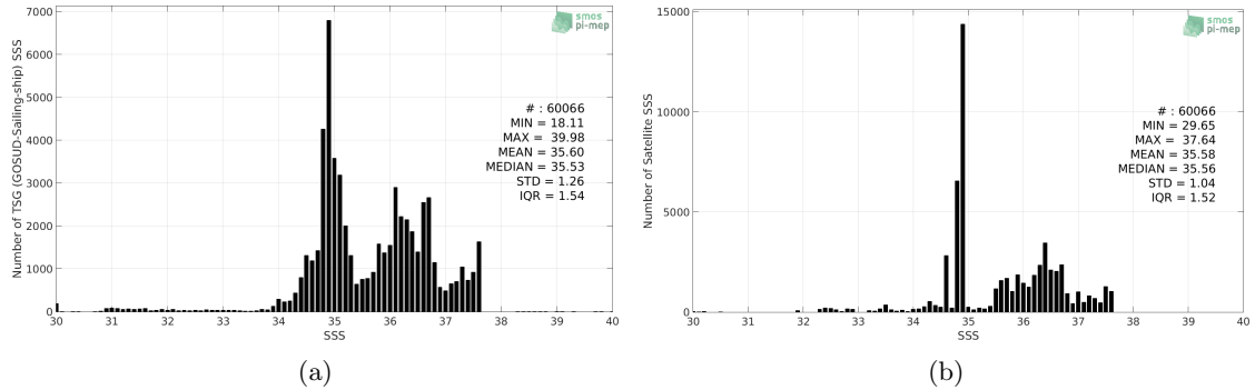
Figure 2: Histograms of SSS from TSG (GOSUD-Sailing-ship) (a) and SMAP SSS L4 OI v1 - 7day (IPRC) (b) considering all match-up pairs per bins of 0.1 over the Amazon and Orinoco river plumes Pi-MEP region and for the full satellite product period.
