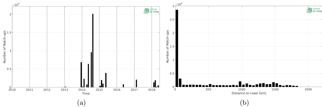
Figure 1: Number of match-ups between TSG (GOSUD-Sailing-ship) and SMAP SSS L4 OI v1 - 7day (IPRC) SSS as a function of time (a) and as function of the distance to coast (b) over the Amazon and Orinoco river plumes Pi-MEP region and for the full satellite product period.
