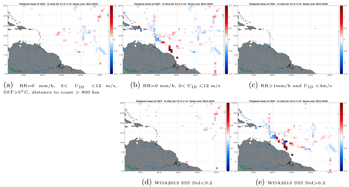
Figure 12: Temporal mean gridded over spatial boxes of size 1°x1° of \Delta SSS (SMAP SSS L4 OI v1 - 7day (IPRC) - TSG (GOSUD-Sailing-ship)) for 5 different subdatasets corresponding to:RR=0 mm/h, 3 < U_{10} < 12 m/s, SST>5°C, distance to coast > 800 km (a), RR=0 mm/h, 3 < U_{10} < 12 m/s (b), RR>1mm/h and U_{10} < 4 m/s (c), WOA2013 SSS Std<0.2 (d), WOA2013 SSS Std>0.2 (e).
