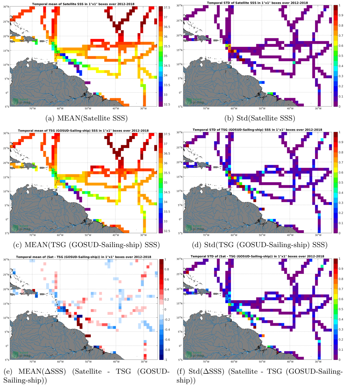
Figure 6: Temporal mean (left) and Std (right) of SSS from SMAP SSS L4 OI v1 - 7day (IPRC) (top), TSG (GOSUD-Sailing-ship) (middle), and of \Delta SSS (Satellite - TSG (GOSUD-Sailing-ship)). Only match-up pairs are used to generate these maps.
