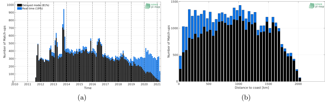
Figure 1: Number of match-ups between Argo and SMAP SSS L4 OI v1 - 7day (IPRC) SSS as a function of time (a) and as function of the distance to coast (b) over the Amazon and Orinoco river plumes Pi-MEP region and for the full satellite product period.
