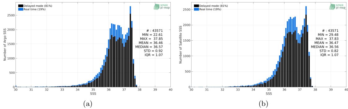
Figure 2: Histograms of SSS from Argo (a) and SMAP SSS L4 OI v1 - 7day (IPRC) (b) considering all match-up pairs per bins of 0.1 over the Amazon and Orinoco river plumes Pi-MEP region and for the full satellite product period.
