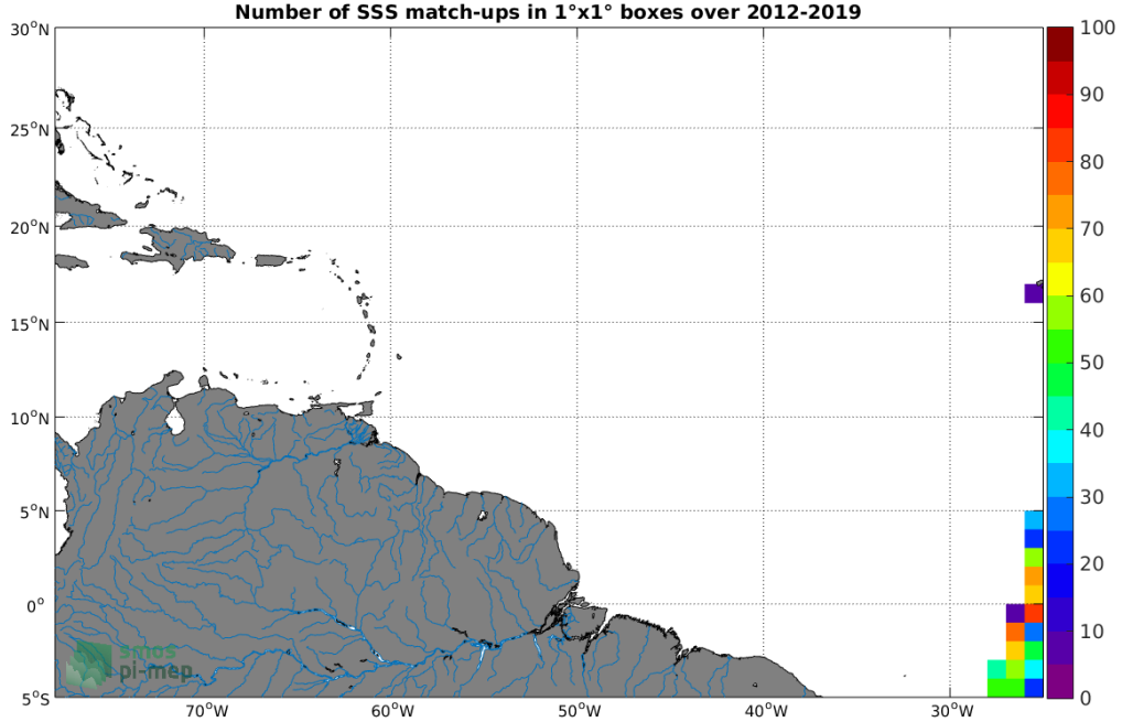
Figure 4: Number of SSS match-ups between TSG (Polarstern) SSS and the SMAP SSS L4 OI v1 - Monthly (IPRC) SSS product for the Amazon and Orinoco river plumes Pi-MEP region over 1^\circ \times 1^\circ boxes and for the full satellite product period.
