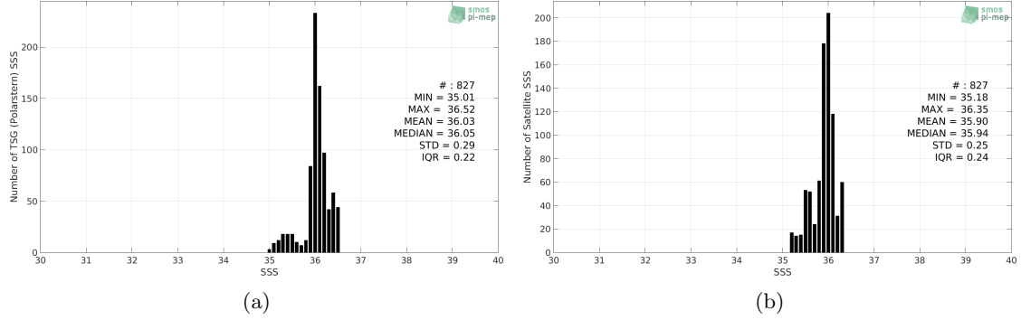
Figure 2: Histograms of SSS from TSG (Polarstern) (a) and SMAP SSS L4 OI v1 - Monthly (IPRC) (b) considering all match-up pairs per bins of 0.1 over the Amazon and Orinoco river plumes Pi-MEP region and for the full satellite product period.
