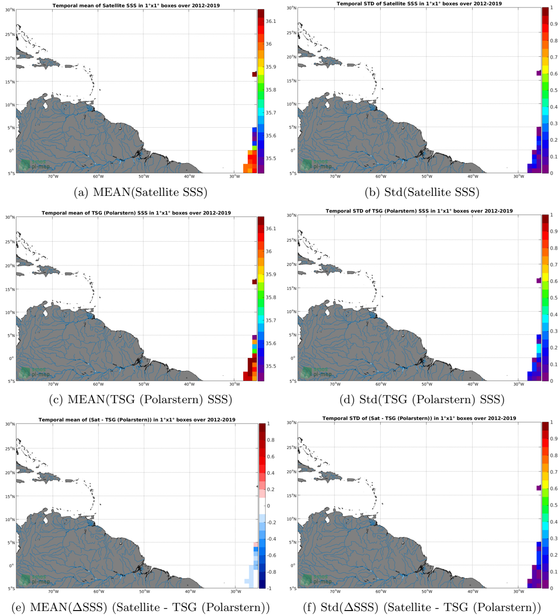
Figure 6: Temporal mean (left) and Std (right) of SSS from SMAP SSS L4 OI v1 - Monthly (IPRC) (top), TSG (Polarstern) (middle), and of \Delta SSS (Satellite - TSG (Polarstern)). Only match-up pairs are used to generate these maps.
