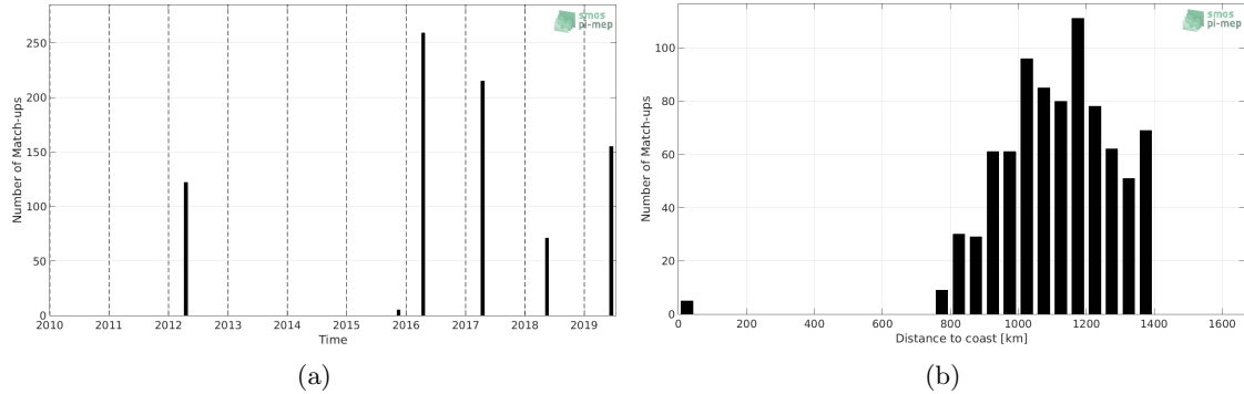
Figure 1: Number of match-ups between TSG (Polarstern) and SMAP SSS L4 OI v1 - Monthly (IPRC) SSS as a function of time (a) and as function of the distance to coast (b) over the Amazon and Orinoco river plumes Pi-MEP region and for the full satellite product period.
