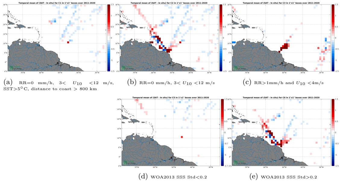
Figure 12: Temporal mean gridded over spatial boxes of size 1^\circ \times 1^\circ of \Delta SSS (SMAP SSS L4 OI v1 - Monthly (IPRC) - TSG (LEGOS-DM)) for 5 different subdatasets corresponding to: RR=0 mm/h, 3 < U_{10} < 12 m/s, SST > 5^\circ C , distance to coast > 800 km (a), RR=0 mm/h, 3 < U_{10} < 12 m/s (b), RR > 1 mm/h and U_{10} < 4 m/s (c), WOA2013 SSS Std < 0.2 (d), WOA2013 SSS Std > 0.2 (e).
