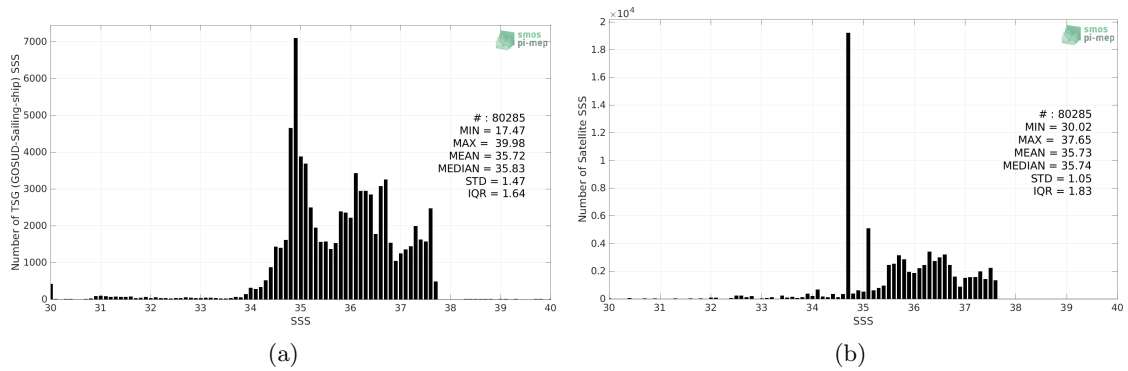
Figure 2: Histograms of SSS from TSG (GOSUD-Sailing-ship) (a) and SMAP SSS L4 OI v1 - Monthly (IPRC) (b) considering all match-up pairs per bins of 0.1 over the Amazon and Orinoco river plumes Pi-MEP region and for the full satellite product period.
