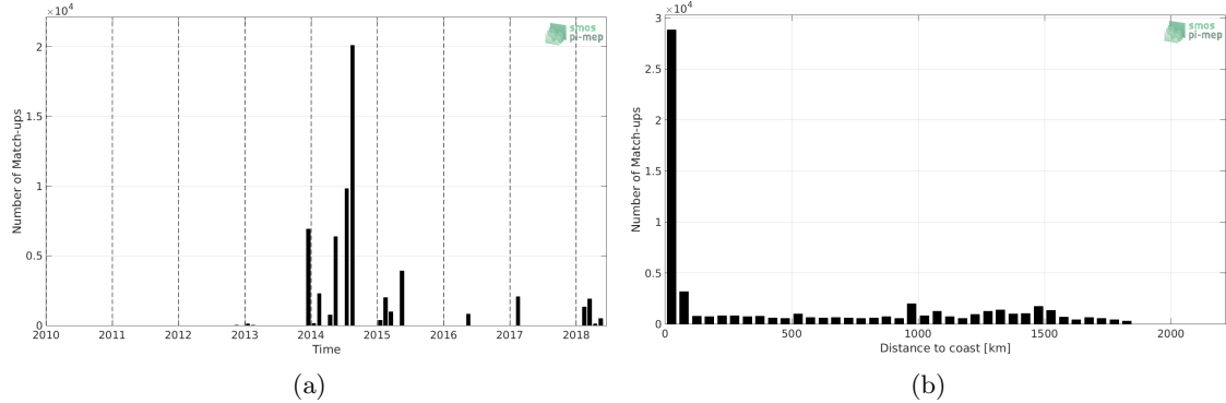
Figure 1: Number of match-ups between TSG (GOSUD-Sailing-ship) and SMAP SSS L4 OI v1 - Monthly (IPRC) SSS as a function of time (a) and as function of the distance to coast (b) over the Amazon and Orinoco river plumes Pi-MEP region and for the full satellite product period.
