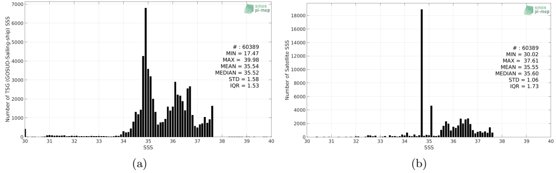
Figure 2: Histograms of SSS from TSG (GOSUD-Sailing-ship) (a) and SMAP SSS L4 OI v1 - Monthly (IPRC) (b) considering all match-up pairs per bins of 0.1 over the Amazon and Orinoco river plumes Pi-MEP region and for the full satellite product period.
