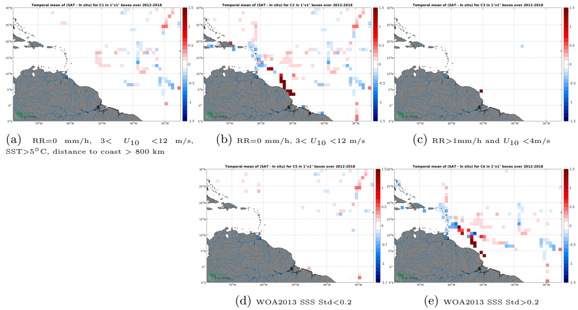
Figure 12: Temporal mean gridded over spatial boxes of size 1^\circ \times 1^\circ of \Delta SSS (SMAP SSS L4 OI v1 - Monthly (IPRC) - TSG (GOSUD-Sailing-ship)) for 5 different subdatasets corresponding to: RR=0 mm/h, 3 < U_{10} < 12 m/s, SST > 5^\circ C , distance to coast > 800 km (a), RR=0 mm/h, 3 < U_{10} < 12 m/s (b), RR > 1 mm/h and U_{10} < 4 m/s (c), WOA2013 SSS Std < 0.2 (d), WOA2013 SSS Std > 0.2 (e).
