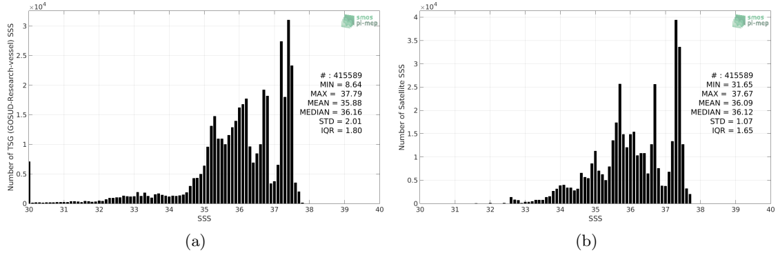
Figure 2: Histograms of SSS from TSG (GOSUD-Research-vessel) (a) and SMAP SSS L4 OI v1 - Monthly (IPRC) (b) considering all match-up pairs per bins of 0.1 over the Amazon and Orinoco river plumes Pi-MEP region and for the full satellite product period.
