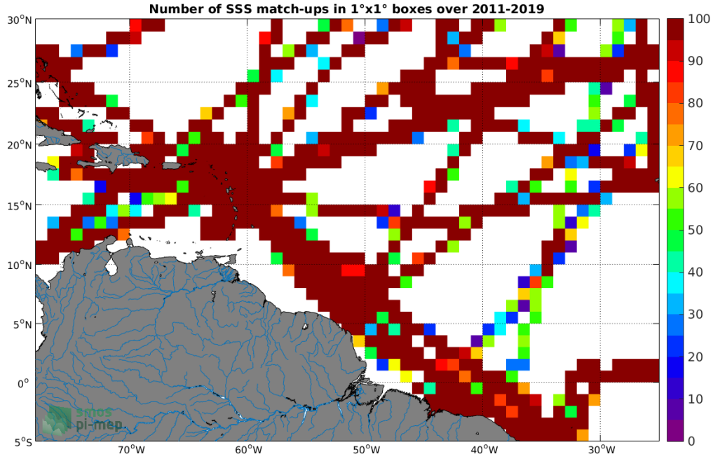
Figure 4: Number of SSS match-ups between TSG (GOSUD-Research-vessel) SSS and the SMAP SSS L4 OI v1 - Monthly (IPRC) SSS product for the Amazon and Orinoco river plumes Pi-MEP region over 1^\circ \times 1^\circ boxes and for the full satellite product period.
