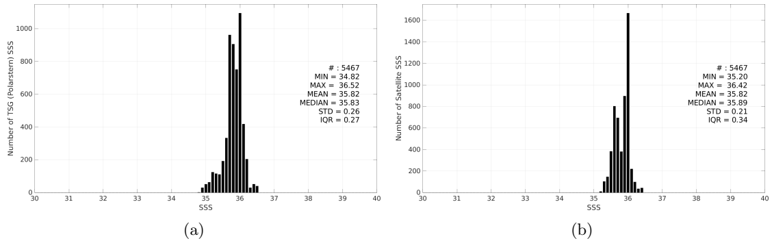
Figure 3: Histograms of SSS from TSG (Polarstern) (a) and SMAP SSS L4 OI v3 - Monthly (ESR) (b) considering all match-up pairs per bins of 0.1 over the Amazon and Orinoco river plumes Pi-MEP region and for the full satellite product period.
