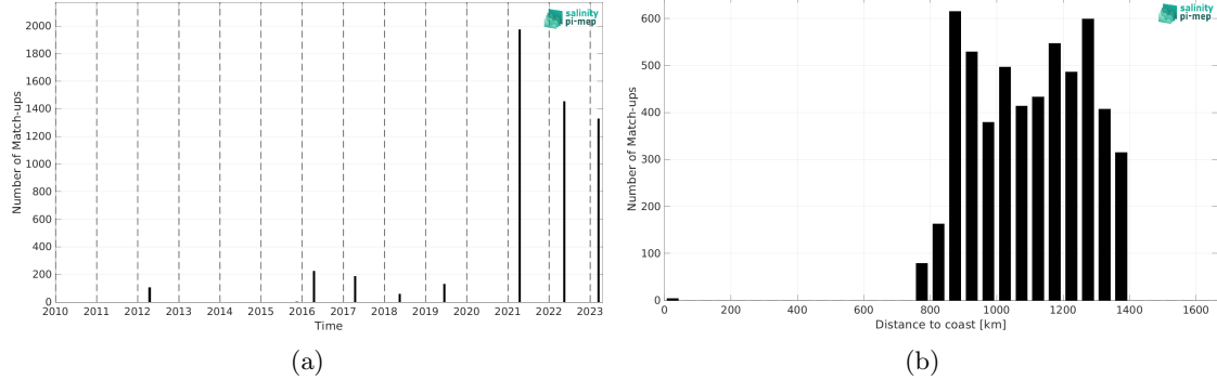
Figure 2: Number of match-ups between TSG (Polarstern) and SMAP SSS L4 OI v3 - Monthly (ESR) SSS as a function of time (a) and as function of the distance to coast (b) over the Amazon and Orinoco river plumes Pi-MEP region and for the full satellite product period.
