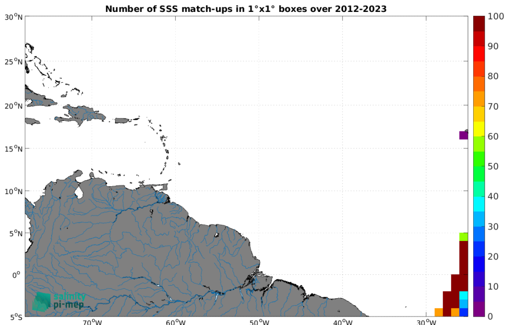
Figure 5: Number of SSS match-ups between TSG (Polarstern) SSS and the SMAP SSS L4 OI v3 - Monthly (ESR) SSS product for the Amazon and Orinoco river plumes Pi-MEP region over 1^\circ \times 1^\circ boxes and for the full satellite product period.
