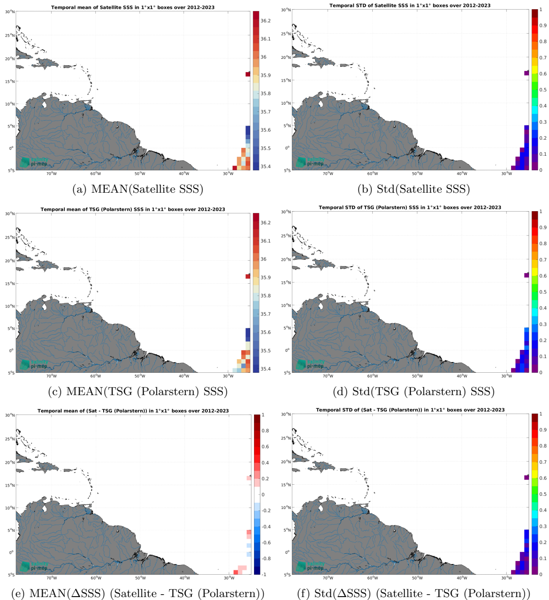
Figure 7: Temporal mean (left) and Std (right) of SSS from SMAP SSS L4 OI v3 - Monthly (ESR) (top), TSG (Polarstern) (middle), and of \Delta SSS (Satellite - TSG (Polarstern)). Only match-up pairs are used to generate these maps.
