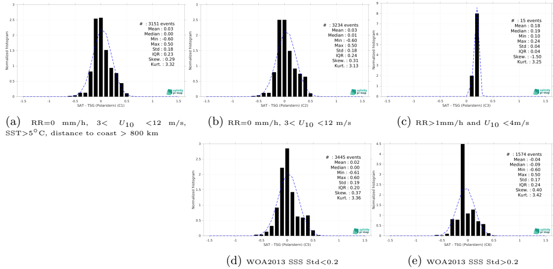
Figure 15: Normalized histogram of \Delta SSS (SMAP SSS L4 OI v3 - Monthly (ESR) - TSG (Polarstern)) for 5 different subdatasets corresponding to: RR=0 mm/h, 3 < U_{10} < 12 m/s, SST > 5°C, distance to coast > 800 km (a), RR=0 mm/h, 3 < U_{10} < 12 m/s (b), RR > 1mm/h and U_{10} < 4 m/s (c), WOA2013 SSS Std < 0.2 (d), WOA2013 SSS Std > 0.2 (e).
