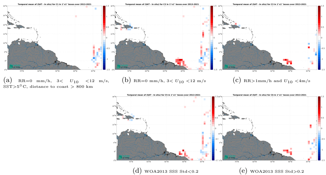
Figure 14: Temporal mean gridded over spatial boxes of size 1^\circ \times 1^\circ of \Delta SSS (SMAP SSS L4 OI v3 - Monthly (ESR) - TSG (CSIC-UTM)) for 5 different subdatasets corresponding to:RR=0 mm/h, 3 < U_{10} < 12 m/s, SST >5^\circ C, distance to coast > 800 km (a), RR=0 mm/h, 3 < U_{10} < 12 m/s (b), RR >1 mm/h and U_{10} < 4 m/s (c), WOA2013 SSS Std <0.2 (d), WOA2013 SSS Std >0.2 (e).
