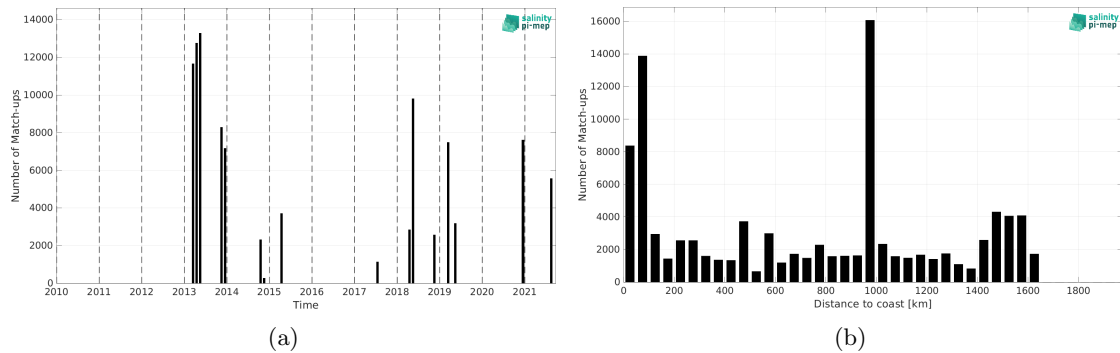
Figure 2: Number of match-ups between TSG (CSIC-UTM) and SMAP SSS L4 OI v3 - Monthly (ESR) SSS as a function of time (a) and as function of the distance to coast (b) over the Amazon and Orinoco river plumes Pi-MEP region and for the full satellite product period.
