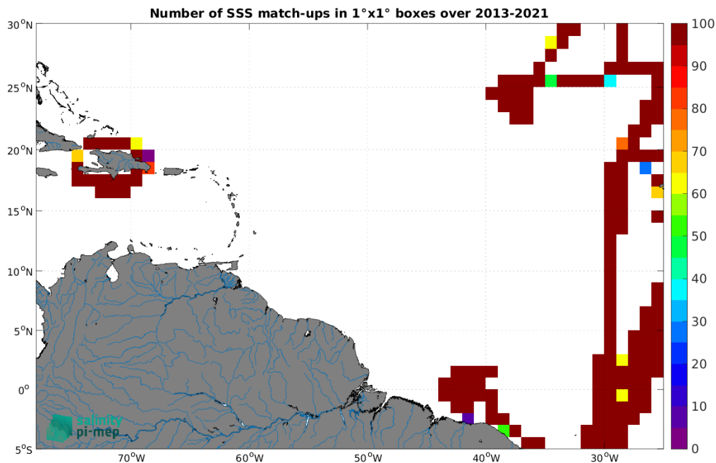
Figure 5: Number of SSS match-ups between TSG (CSIC-UTM) SSS and the SMAP SSS L4 OI v3 - Monthly (ESR) SSS product for the Amazon and Orinoco river plumes Pi-MEP region over 1^\circ \times 1^\circ boxes and for the full satellite product period.
