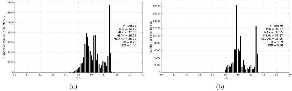
Figure 3: Histograms of SSS from TSG (CSIC-UTM) (a) and SMAP SSS L4 OI v3 - Monthly (ESR) (b) considering all match-up pairs per bins of 0.1 over the Amazon and Orinoco river plumes Pi-MEP region and for the full satellite product period.
