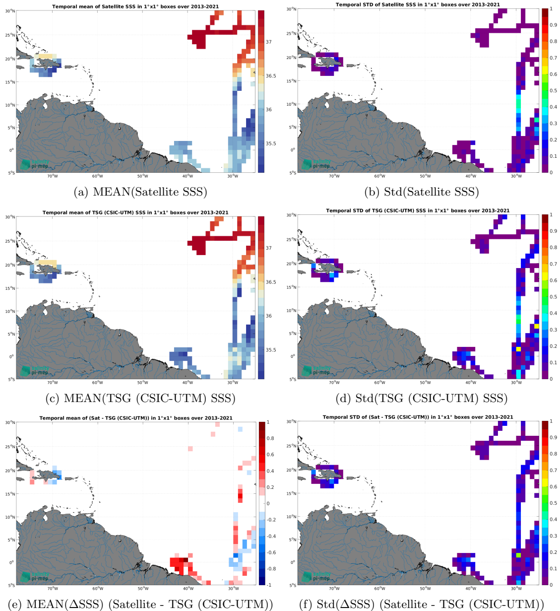
Figure 7: Temporal mean (left) and Std (right) of SSS from SMAP SSS L4 OI v3 - Monthly (ESR) (top), TSG (CSIC-UTM) (middle), and of \Delta SSS (Satellite - TSG (CSIC-UTM)). Only match-up pairs are used to generate these maps.
