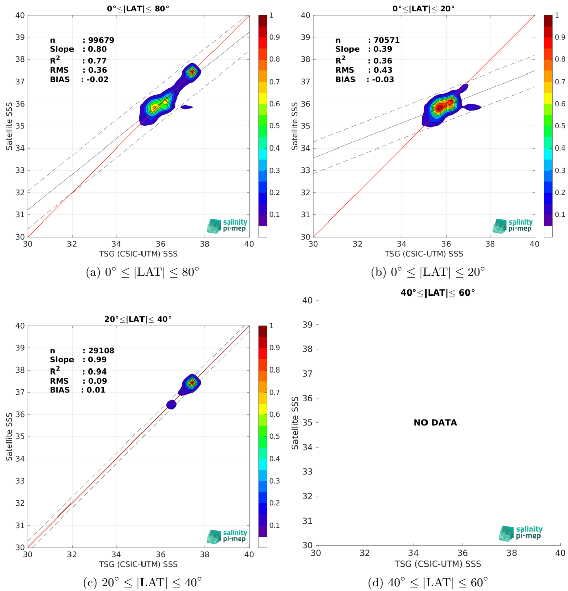
Figure 10: Contour maps of the concentration of SMAP SSS L4 OI v3 - Monthly (ESR) SSS (y-axis) versus TSG (CSIC-UTM) SSS (x-axis) at match-up pairs for different latitude bands. For each plot, the red line shows x=y . The black thin and dashed lines indicate a linear fit through the data cloud and the \pm 95\% confidence levels, respectively. The number match-up pairs n , the slope and R^2 coefficient of the linear fit, the root mean square (RMS) and the mean bias between satellite and in situ data are indicated for each latitude band in each plots.
