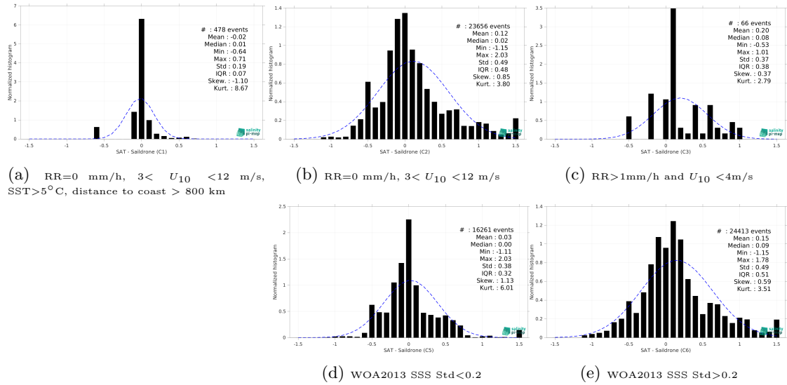
Figure 15: Normalized histogram of \Delta\text{SSS} (SMAP SSS L4 OI v3 - Monthly (ESR) - Saldrone) for 5 different subdatasets corresponding to: RR=0 mm/h, 3 < U_{10} < 12 m/s, SST >5^{\circ}\text{C} , distance to coast > 800 km (a), RR=0 mm/h, 3 < U_{10} < 12 m/s (b), RR>1\text{mm/h} and U_{10} < 4\text{m/s} (c), WOA2013 SSS Std <0.2 (d), WOA2013 SSS Std >0.2 (e).
