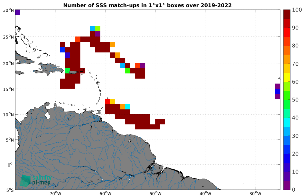
Figure 5: Number of SSS match-ups between Saildrone SSS and the SMAP SSS L4 OI v3 - Monthly (ESR) SSS product for the Amazon and Orinoco river plumes Pi-MEP region over 1^\circ \times 1^\circ boxes and for the full satellite product period.
