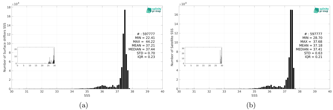
Figure 3: Histograms of SSS from Surface drifters (a) and SMAP SSS L4 OI v3 - Monthly (ESR) (b) considering all match-up pairs per bins of 0.1 over the Amazon and Orinoco river plumes Pi-MEP region and for the full satellite product period.
