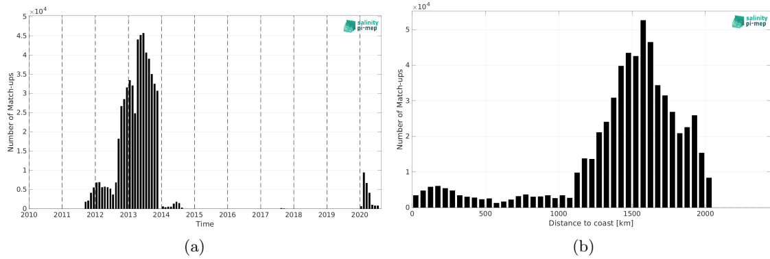
Figure 2: Number of match-ups between Surface drifters and SMAP SSS L4 OI v3 - Monthly (ESR) SSS as a function of time (a) and as function of the distance to coast (b) over the Amazon and Orinoco river plumes Pi-MEP region and for the full satellite product period.
