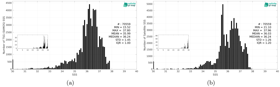
Figure 3: Histograms of SSS from TSG (SAMOS) (a) and SMAP SSS L4 OI v3 - Daily (ESR) (b) considering all match-up pairs per bins of 0.1 over the Amazon and Orinoco river plumes Pi-MEP region and for the full satellite product period.
