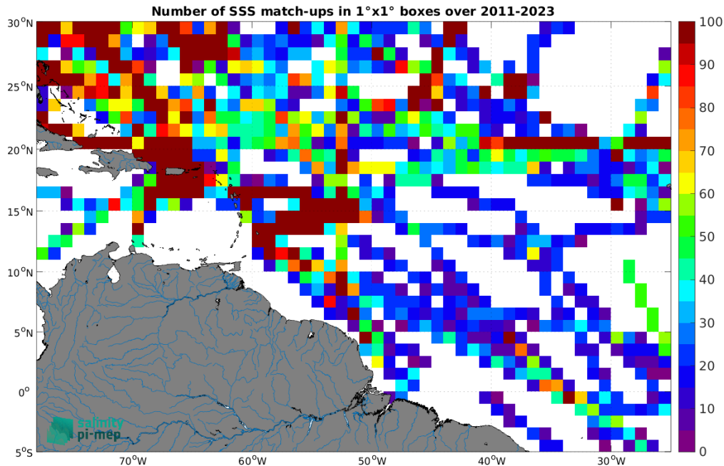
Figure 5: Number of SSS match-ups between TSG (SAMOS) SSS and the SMAP SSS L4 OI v3 - Daily (ESR) SSS product for the Amazon and Orinoco river plumes Pi-MEP region over 1^{\circ} \times 1^{\circ} boxes and for the full satellite product period.
