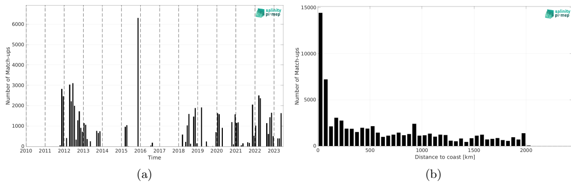
Figure 2: Number of match-ups between TSG (SAMOS) and SMAP SSS L4 OI v3 - Daily (ESR) SSS as a function of time (a) and as function of the distance to coast (b) over the Amazon and Orinoco river plumes Pi-MEP region and for the full satellite product period.
