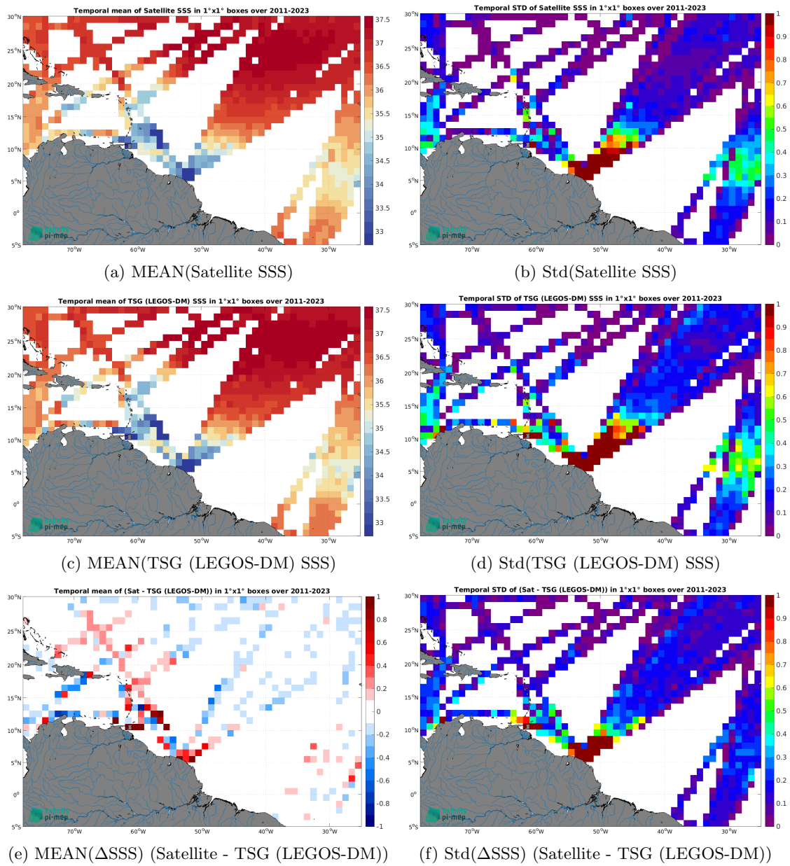
Figure 7: Temporal mean (left) and Std (right) of SSS from SMAP SSS L4 OI v3 - Daily (ESR) (top), TSG (LEGOS-DM) (middle), and of \Delta SSS (Satellite - TSG (LEGOS-DM)). Only match-up pairs are used to generate these maps.
