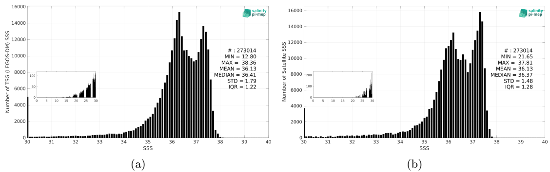
Figure 3: Histograms of SSS from TSG (LEGOS-DM) (a) and SMAP SSS L4 OI v3 - Daily (ESR) (b) considering all match-up pairs per bins of 0.1 over the Amazon and Orinoco river plumes Pi-MEP region and for the full satellite product period.
