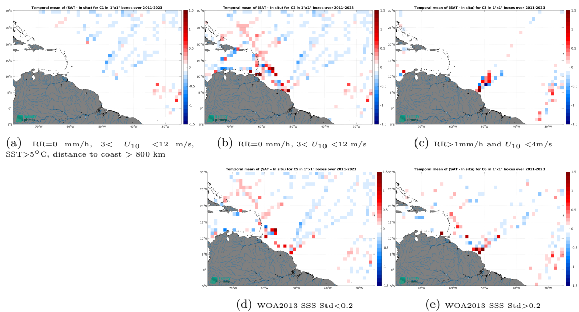
Figure 14: Temporal mean gridded over spatial boxes of size 1^\circ \times 1^\circ of \Delta SSS (SMAP SSS L4 OI v3 - Daily (ESR) - TSG (LEGOS-DM)) for 5 different subdatasets corresponding to:RR=0 mm/h, 3 < U_{10} < 12 m/s, SST >5^\circ\text{C} , distance to coast > 800 km (a), RR=0 mm/h, 3 < U_{10} < 12 m/s (b), RR >1 mm/h and U_{10} < 4 m/s (c), WOA2013 SSS Std <0.2 (d), WOA2013 SSS Std >0.2 (e).
