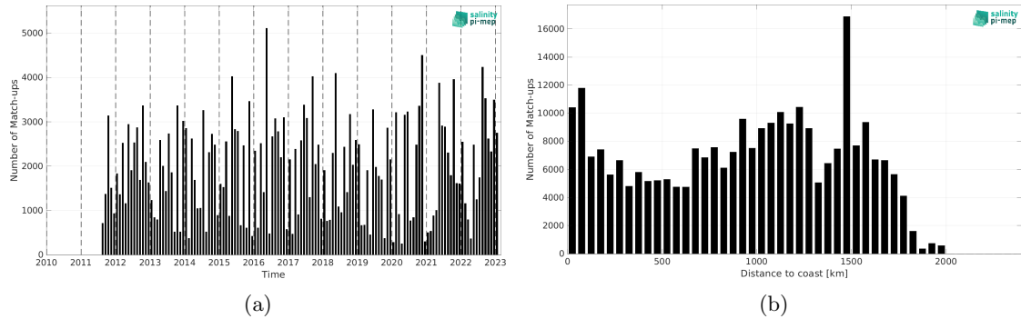
Figure 2: Number of match-ups between TSG (LEGOS-DM) and SMAP SSS L4 OI v3 - Daily (ESR) SSS as a function of time (a) and as function of the distance to coast (b) over the Amazon and Orinoco river plumes Pi-MEP region and for the full satellite product period.
