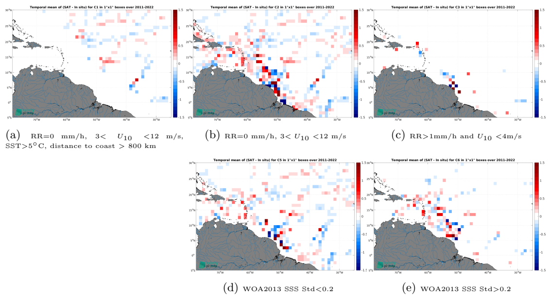
Figure 14: Temporal mean gridded over spatial boxes of size 1^\circ \times 1^\circ of \Delta SSS (SMAP SSS L4 OI v3 - Daily (ESR) - TSG (GOSUD-Research-vessel)) for 5 different subdatasets corresponding to:RR=0 mm/h, 3 < U_{10} < 12 m/s, SST >5^\circ C, distance to coast > 800 km (a), RR=0 mm/h, 3 < U_{10} < 12 m/s (b), RR >1 mm/h and U_{10} < 4 m/s (c), WOA2013 SSS Std <0.2 (d), WOA2013 SSS Std >0.2 (e).
