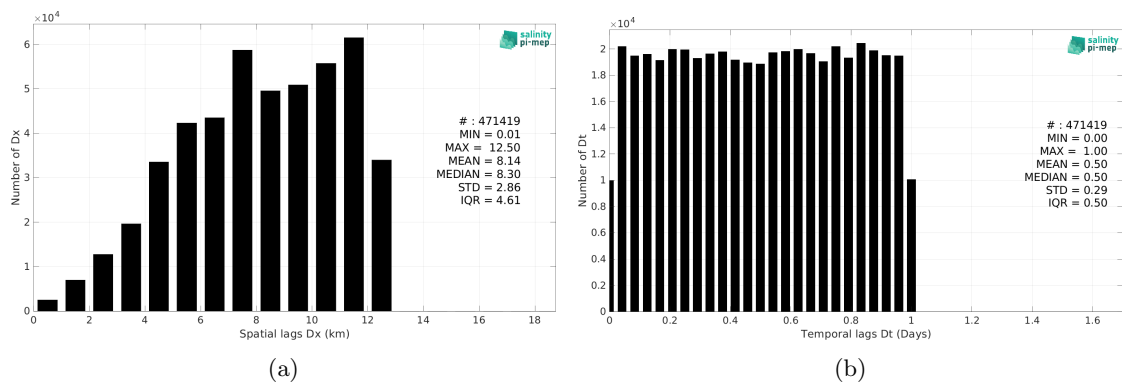
Figure 6: Histograms of the spatial (a) and temporal (b) lags between the location/time of the TSG (GOSUD-Research-vessel) measurement and the date of the corresponding SMAP SSS L4 OI v3 - Daily (ESR) SSS pixel.
