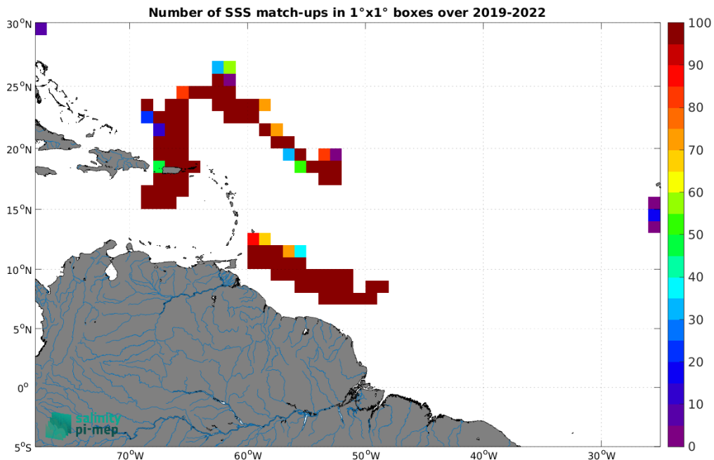
Figure 5: Number of SSS match-ups between Saildrone SSS and the SMAP SSS L4 OI v3 - Daily (ESR) SSS product for the Amazon and Orinoco river plumes Pi-MEP region over 1^\circ \times 1^\circ boxes and for the full satellite product period.
