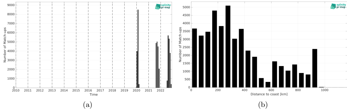
Figure 2: Number of match-ups between Saildrone and SMAP SSS L4 OI v3 - Daily (ESR) SSS as a function of time (a) and as function of the distance to coast (b) over the Amazon and Orinoco river plumes Pi-MEP region and for the full satellite product period.
