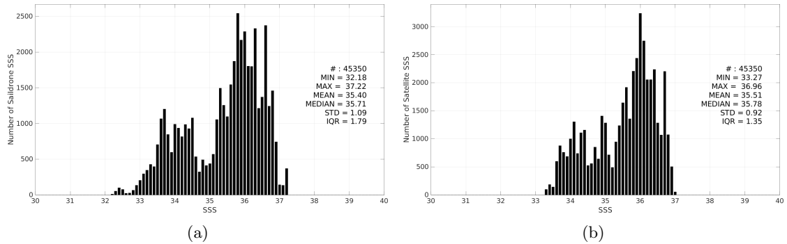
Figure 3: Histograms of SSS from Saildrone (a) and SMAP SSS L4 OI v3 - Daily (ESR) (b) considering all match-up pairs per bins of 0.1 over the Amazon and Orinoco river plumes Pi-MEP region and for the full satellite product period.
