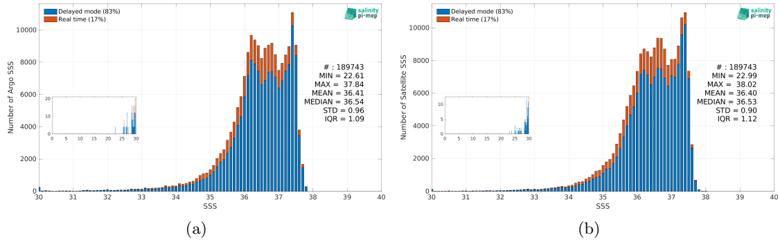
Figure 3: Histograms of SSS from Argo (a) and SMAP SSS L4 OI v3 - Daily (ESR) (b) considering all match-up pairs per bins of 0.1 over the Amazon and Orinoco river plumes Pi-MEP region and for the full satellite product period.
