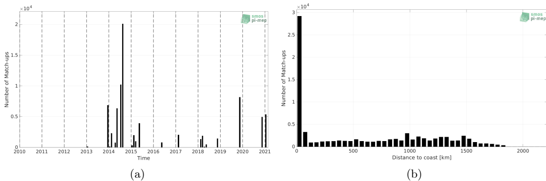
Figure 1: Number of match-ups between TSG (GOSUD-Sailing-ship) and SMAP SSS L4 OI v2 - 7 Days (ESR) SSS as a function of time (a) and as function of the distance to coast (b) over the Amazon and Orinoco river plumes Pi-MEP region and for the full satellite product period.
