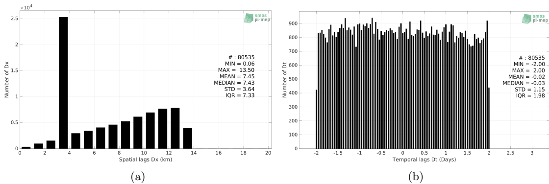
Figure 5: Histograms of the spatial (a) and temporal (b) lags between the location/time of the TSG (GOSUD-Sailing-ship) measurement and the date of the corresponding SMAP SSS L4 OI v2 - 7 Days (ESR) SSS pixel.
