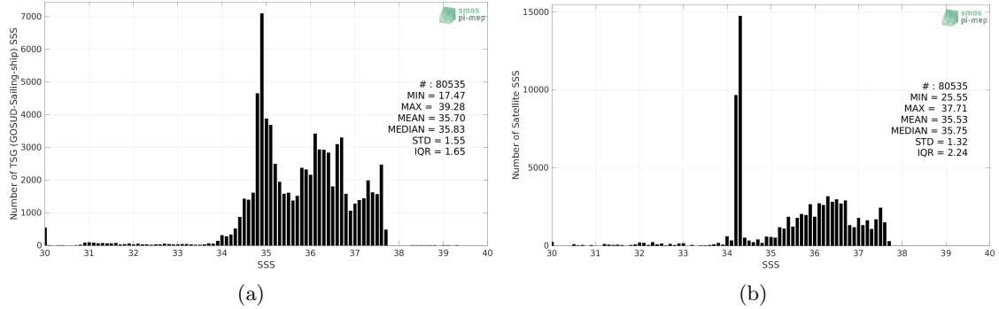
Figure 2: Histograms of SSS from TSG (GOSUD-Sailing-ship) (a) and SMAP SSS L4 OI v2 - 7 Days (ESR) (b) considering all match-up pairs per bins of 0.1 over the Amazon and Orinoco river plumes Pi-MEP region and for the full satellite product period.
