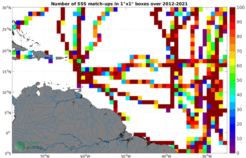
Figure 4: Number of SSS match-ups between TSG (GOSUD-Sailing-ship) SSS and the SMAP SSS L4 OI v2 - 7 Days (ESR) SSS product for the Amazon and Orinoco river plumes Pi-MEP region over 1^\circ \times 1^\circ boxes and for the full satellite product period.
