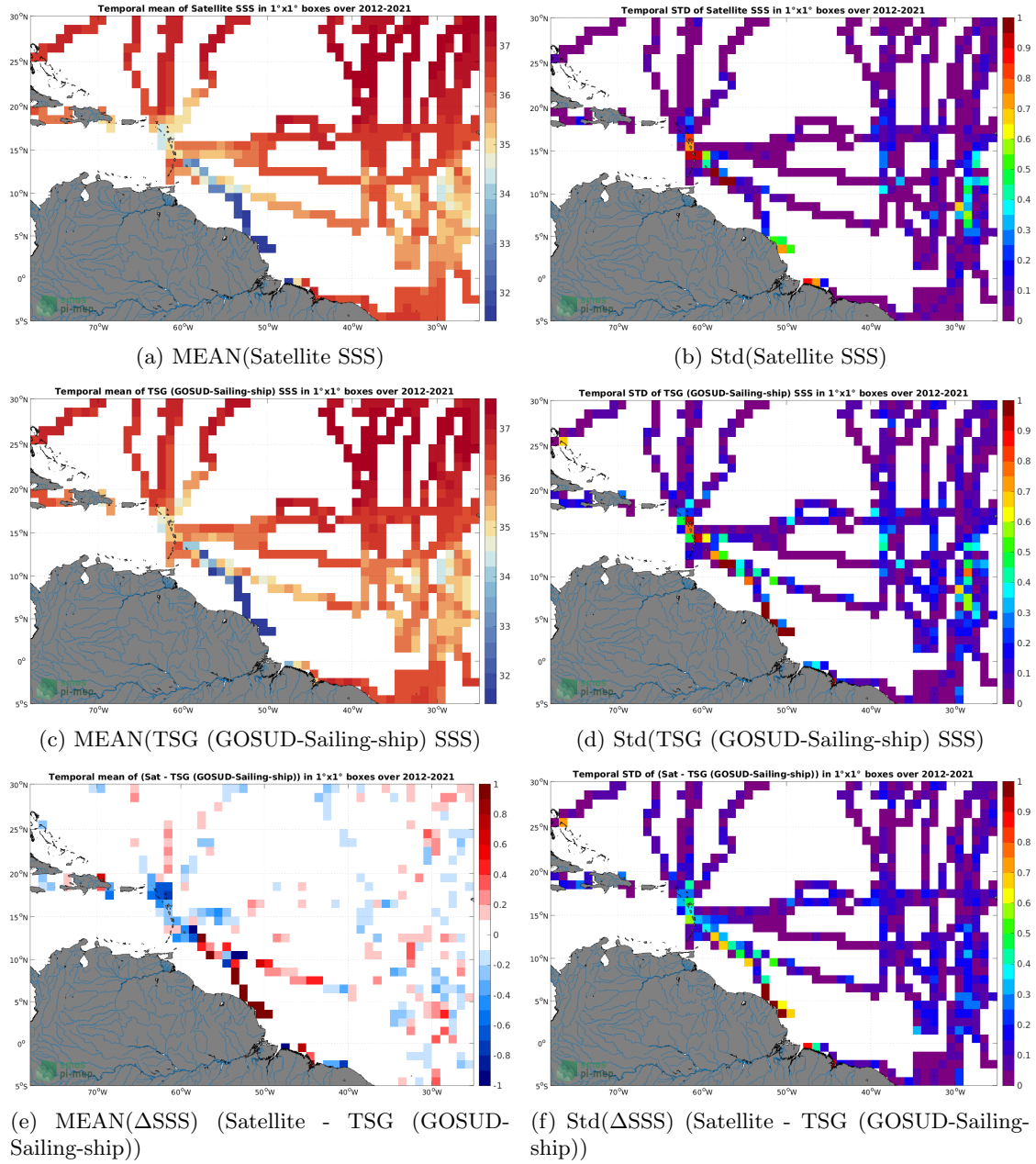
Figure 6: Temporal mean (left) and Std (right) of SSS from SMAP SSS L4 OI v2 - 7 Days (ESR) (top), TSG (GOSUD-Sailing-ship) (middle), and of \Delta SSS (Satellite - TSG (GOSUD-Sailing-ship)). Only match-up pairs are used to generate these maps.
