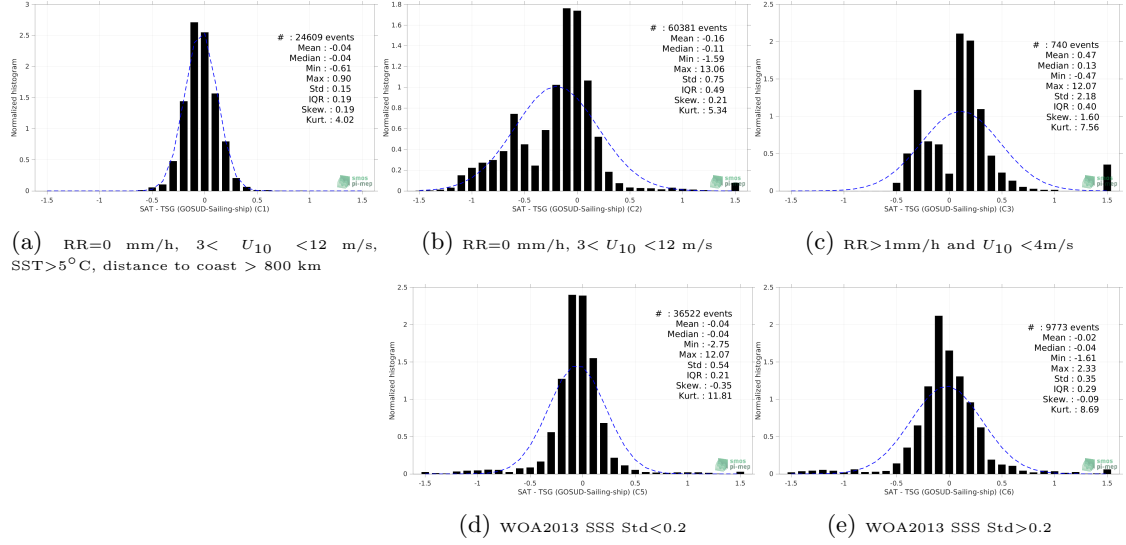
Figure 13: Normalized histogram of \Delta SSS (SMAP SSS L4 OI v2 - 7 Days (ESR) - TSG (GOSUD-Sailing-ship)) for 5 different subdatasets corresponding to: RR=0 mm/h, 3 < U_{10} < 12 m/s, SST > 5°C, distance to coast > 800 km (a), RR=0 mm/h, 3 < U_{10} < 12 m/s (b), RR > 1mm/h and U_{10} < 4 m/s (c), WOA2013 SSS Std < 0.2 (d), WOA2013 SSS Std > 0.2 (e).
