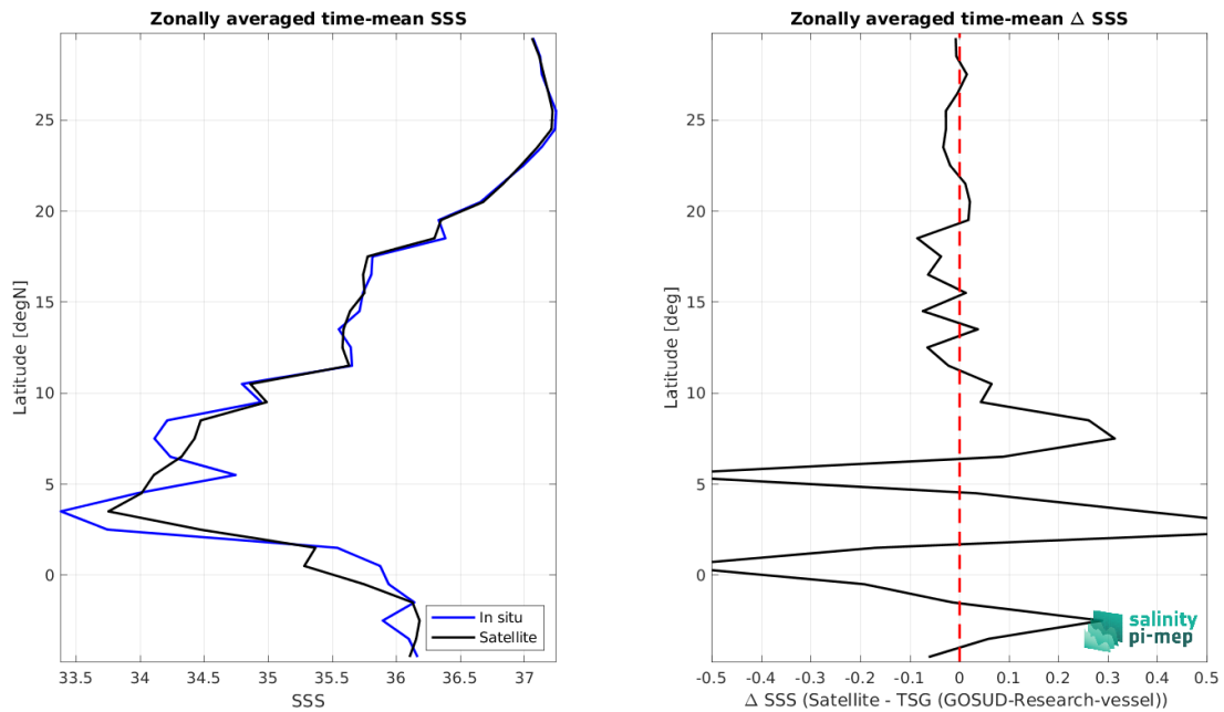
Figure 8: Left panel: Zonal mean SSS from SMAP SSS L4 OI v2 - 7 Days (ESR) satellite product (black) and from TSG (GOSUD-Research-vessel) (blue). Right panel: Zonal mean of \Delta SSS (Satellite - TSG (GOSUD-Research-vessel)) for all the collected Pi-MEP match-up pairs estimated over the full satellite product period.
