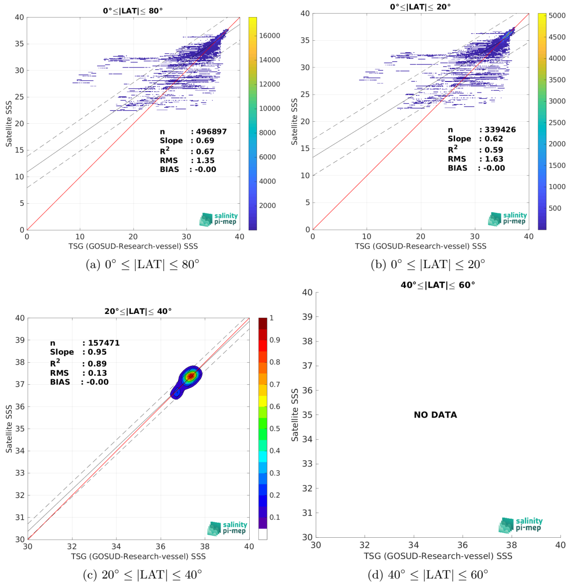
Figure 9: Contour maps of the concentration of SMAP SSS L4 OI v2 - 7 Days (ESR) SSS (y-axis) versus TSG (GOSUD-Research-vessel) SSS (x-axis) at match-up pairs for different latitude bands. For each plot, the red line shows x=y . The black thin and dashed lines indicate a linear fit through the data cloud and the \pm 95\% confidence levels, respectively. The number match-up pairs n , the slope and R^2 coefficient of the linear fit, the root mean square (RMS) and the mean bias between satellite and in situ data are indicated for each latitude band in each plots.
