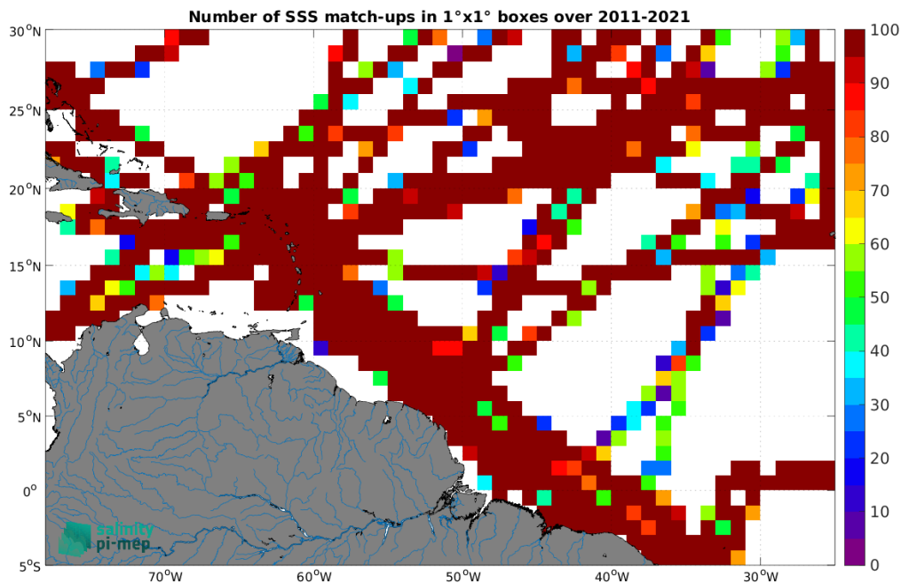
Figure 4: Number of SSS match-ups between TSG (GOSUD-Research-vessel) SSS and the SMAP SSS L4 OI v2 - 7 Days (ESR) SSS product for the Amazon and Orinoco river plumes Pi-MEP region over 1^\circ \times 1^\circ boxes and for the full satellite product period.
