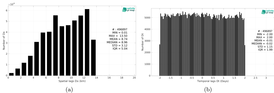
Figure 5: Histograms of the spatial (a) and temporal (b) lags between the location/time of the TSG (GOSUD-Research-vessel) measurement and the date of the corresponding SMAP SSS L4 OI v2 - 7 Days (ESR) SSS pixel.
