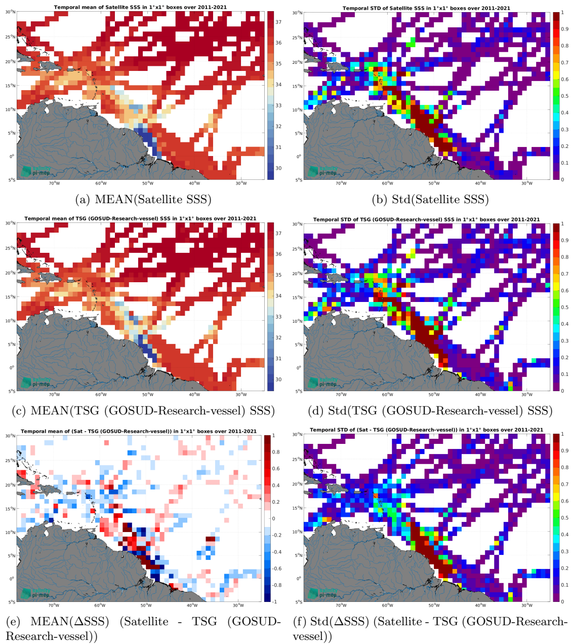
Figure 6: Temporal mean (left) and Std (right) of SSS from SMAP SSS L4 OI v2 - 7 Days (ESR) (top), TSG (GOSUD-Research-vessel) (middle), and of \Delta SSS (Satellite - TSG (GOSUD-Research-vessel)). Only match-up pairs are used to generate these maps.
