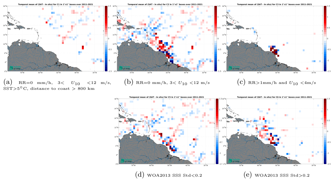
Figure 12: Temporal mean gridded over spatial boxes of size 1^\circ \times 1^\circ of \Delta\text{SSS} (SMAP SSS L4 OI v2 - 7 Days (ESR) - TSG (GOSUD-Research-vessel)) for 5 different subdatasets corresponding to:RR=0 mm/h, 3 < U_{10} < 12 m/s, SST >5^\circ\text{C} , distance to coast > 800 km (a), RR=0 mm/h, 3 < U_{10} < 12 m/s (b), RR >1 mm/h and U_{10} < 4 m/s (c), WOA2013 SSS Std <0.2 (d), WOA2013 SSS Std >0.2 (e).
