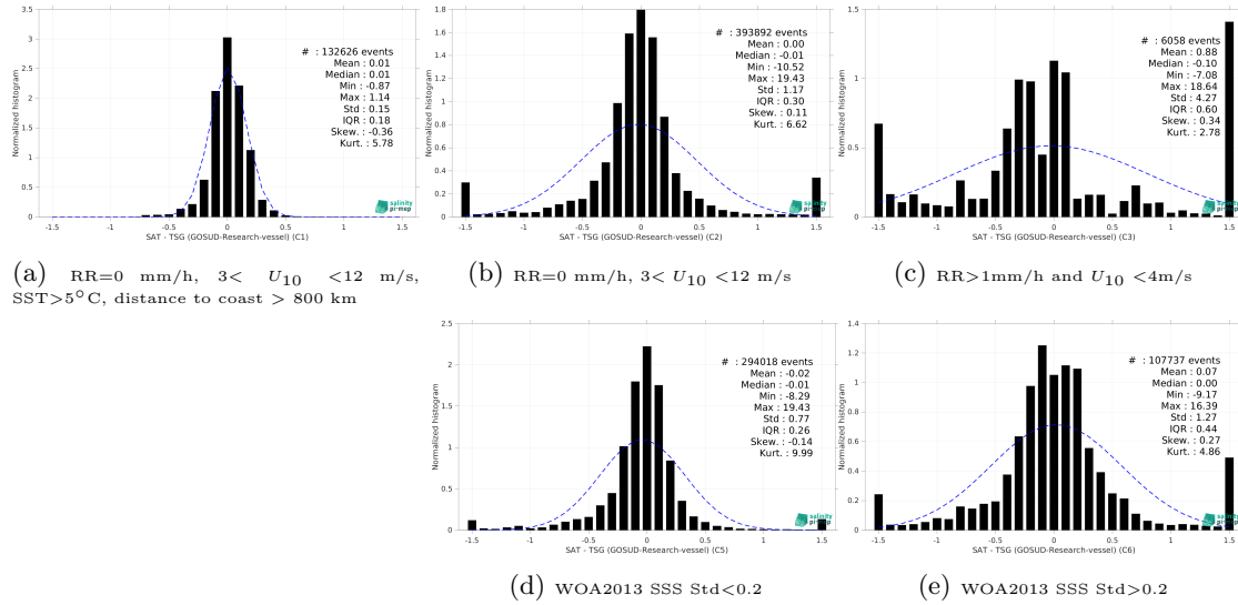
Figure 13: Normalized histogram of \Delta SSS (SMAP SSS L4 OI v2 - 7 Days (ESR) - TSG (GOSUD-Research-vessel)) for 5 different subdatasets corresponding to: RR=0 mm/h, 3 < U_{10} < 12 m/s, SST > 5°C, distance to coast > 800 km (a), RR=0 mm/h, 3 < U_{10} < 12 m/s (b), RR > 1mm/h and U_{10} < 4 m/s (c), WOA2013 SSS Std < 0.2 (d), WOA2013 SSS Std > 0.2 (e).
