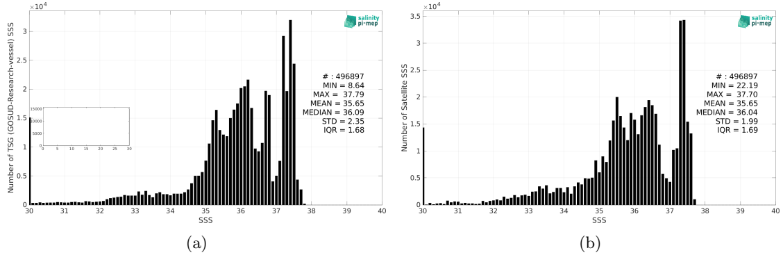
Figure 2: Histograms of SSS from TSG (GOSUD-Research-vessel) (a) and SMAP SSS L4 OI v2 - 7 Days (ESR) (b) considering all match-up pairs per bins of 0.1 over the Amazon and Orinoco river plumes Pi-MEP region and for the full satellite product period.
