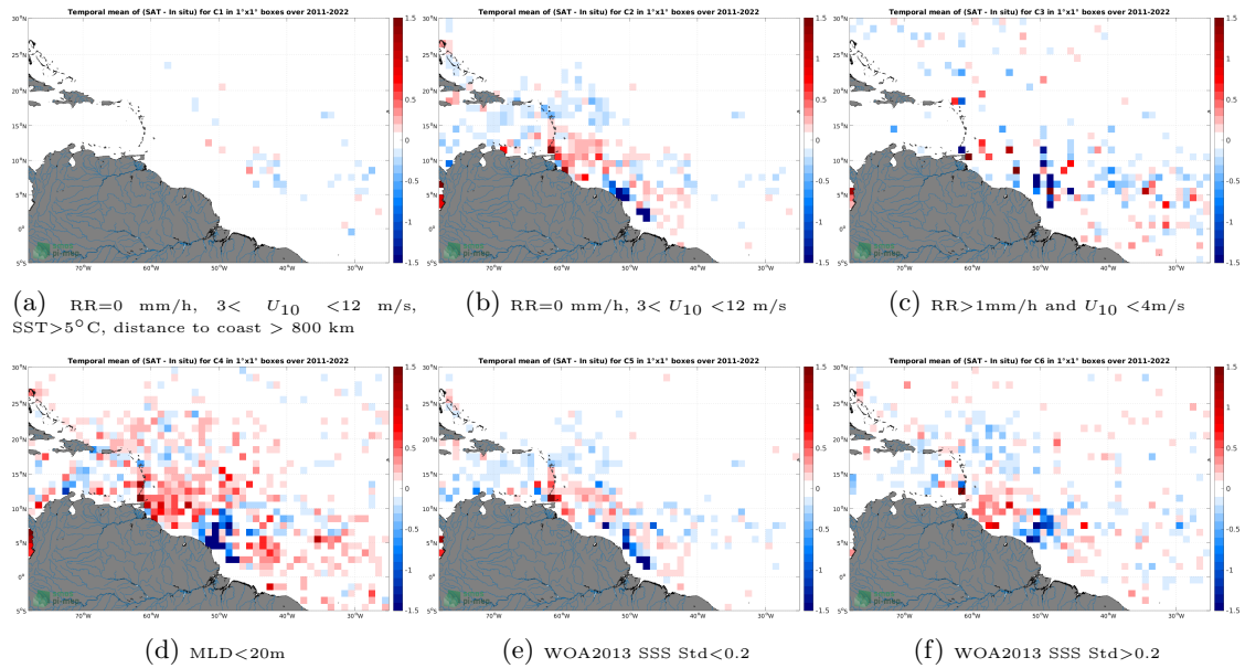
Figure 12: Temporal mean gridded over spatial boxes of size 1^\circ \times 1^\circ of \Delta SSS (SMAP SSS L4 OI v2 - 7 Days (ESR) - Argo) for 6 different subdatasets corresponding to:RR=0 mm/h, 3 < U_{10} < 12 m/s, SST >5^\circ C, distance to coast > 800 km (a), RR=0 mm/h, 3 < U_{10} < 12 m/s (b), RR >1 mm/h and U_{10} < 4 m/s (c),MLD <20 m (d),WOA2013 SSS Std <0.2 (e),WOA2013 SSS Std >0.2 (f).
