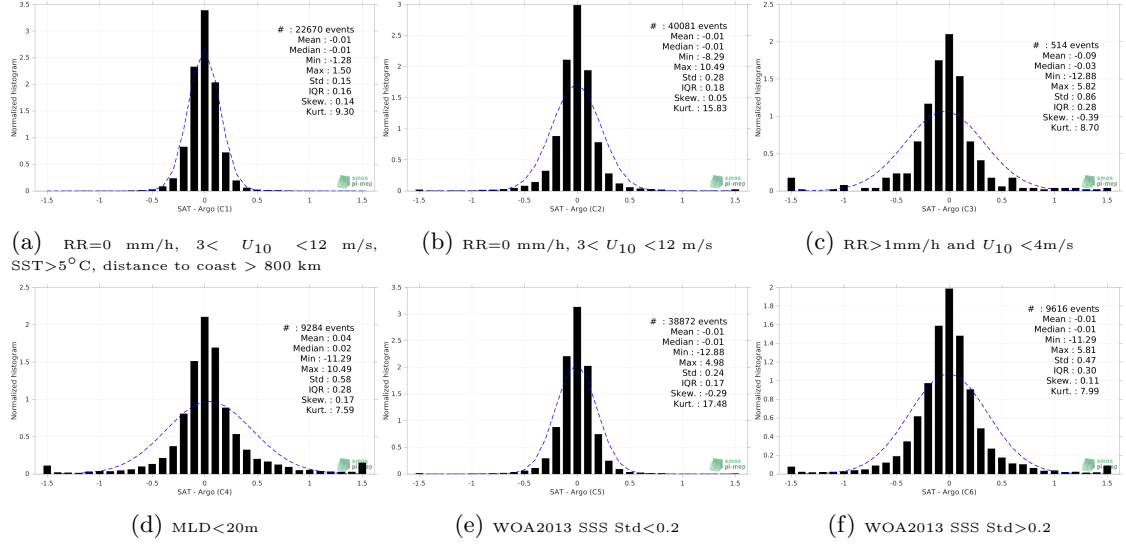
Figure 13: Normalized histogram of \Delta SSS (SMAP SSS L4 OI v2 - 7 Days (ESR) - Argo) for 6 different subdatasets corresponding to: RR=0 mm/h, 3 < U_{10} < 12 m/s, SST>5°C, distance to coast > 800 km (a), RR=0 mm/h, 3 < U_{10} < 12 m/s (b), RR>1mm/h and U_{10} < 4 m/s (c), MLD<20m (d), WOA2013 SSS Std<0.2 (e), WOA2013 SSS Std>0.2 (f).
