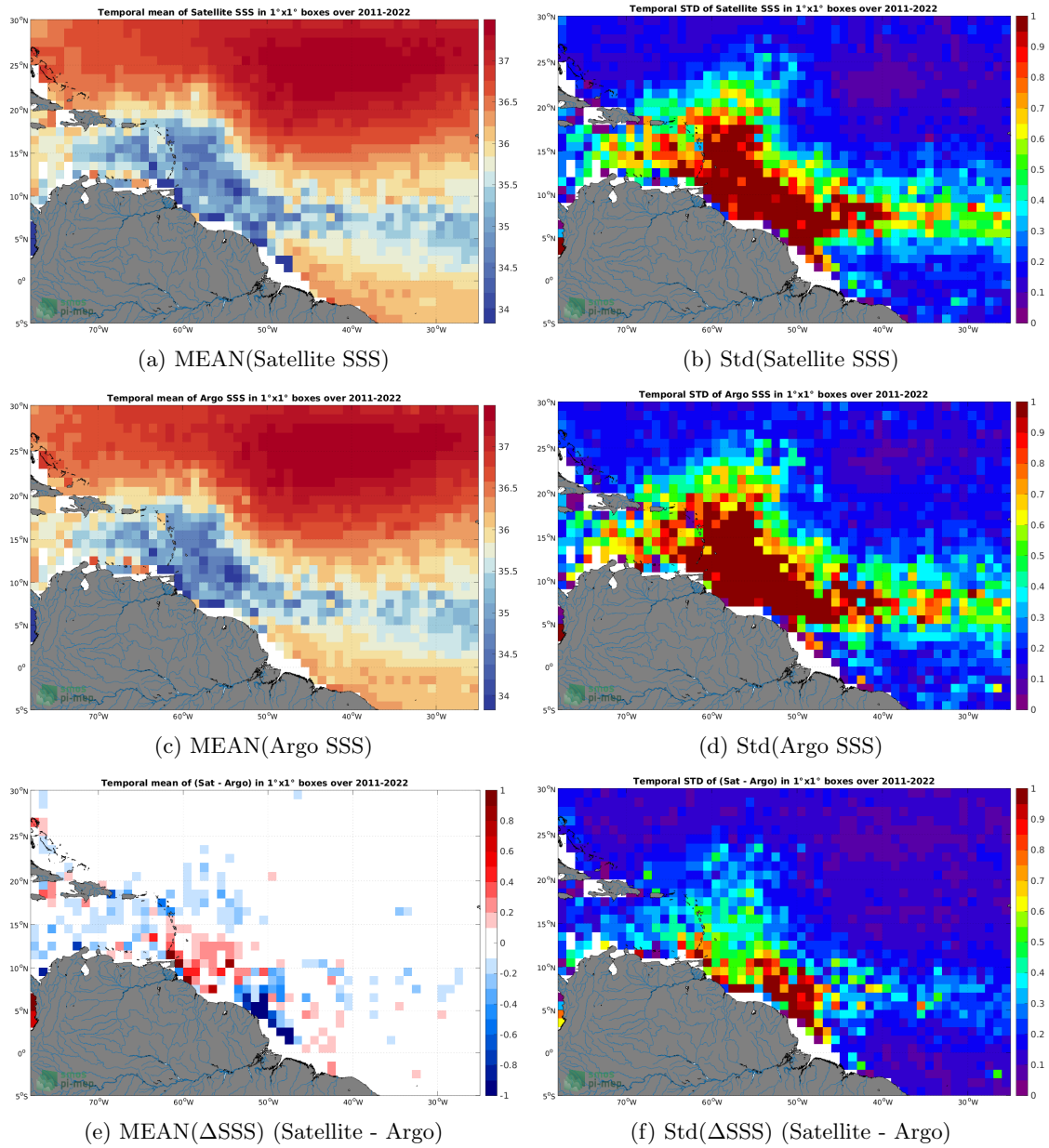
Figure 6: Temporal mean (left) and Std (right) of SSS from SMAP SSS L4 OI v2 - 7 Days (ESR) (top), Argo (middle), and of \Delta SSS (Satellite - Argo). Only match-up pairs are used to generate these maps.
