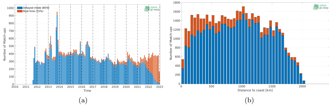
Figure 1: Number of match-ups between Argo and SMAP SSS L4 OI v2 - 7 Days (ESR) SSS as a function of time (a) and as function of the distance to coast (b) over the Amazon and Orinoco river plumes Pi-MEP region and for the full satellite product period.
