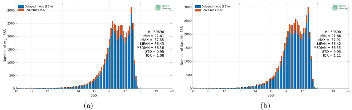
Figure 2: Histograms of SSS from Argo (a) and SMAP SSS L4 OI v2 - 7 Days (ESR) (b) considering all match-up pairs per bins of 0.1 over the Amazon and Orinoco river plumes Pi-MEP region and for the full satellite product period.
