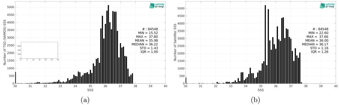
Figure 2: Histograms of SSS from TSG (SAMOS) (a) and SMAP SSS L4 OI v2 - Monthly (IPRC) (b) considering all match-up pairs per bins of 0.1 over the Amazon and Orinoco river plumes Pi-MEP region and for the full satellite product period.
