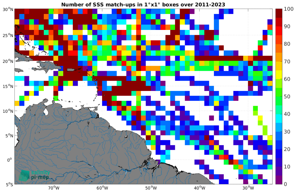
Figure 4: Number of SSS match-ups between TSG (SAMOS) SSS and the SMAP SSS L4 OI v2 - Monthly (IPRC) SSS product for the Amazon and Orinoco river plumes Pi-MEP region over 1°×1° boxes and for the full satellite product period.
