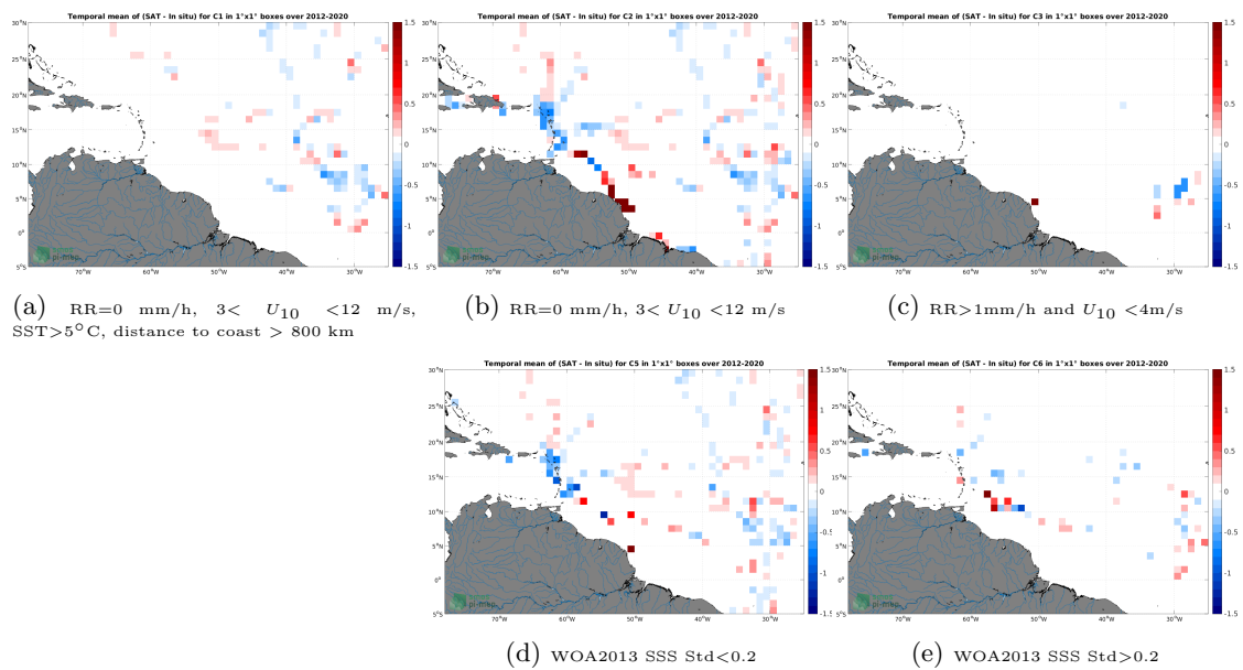
Figure 12: Temporal mean gridded over spatial boxes of size 1^\circ \times 1^\circ of \Delta SSS (SMAP SSS L4 OI v2 - Monthly (IPRC) - TSG (GOSUD-Sailing-ship)) for 5 different subdatasets corresponding to: RR=0 mm/h, 3 < U_{10} < 12 m/s, SST > 5°C, distance to coast > 800 km (a), RR=0 mm/h, 3 < U_{10} < 12 m/s (b), RR > 1mm/h and U_{10} < 4 m/s (c), WOA2013 SSS Std < 0.2 (d), WOA2013 SSS Std > 0.2 (e).
