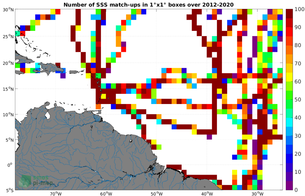
Figure 4: Number of SSS match-ups between TSG (GOSUD-Sailing-ship) SSS and the SMAP SSS L4 OI v2 - Monthly (IPRC) SSS product for the Amazon and Orinoco river plumes Pi-MEP region over 1^\circ \times 1^\circ boxes and for the full satellite product period.
