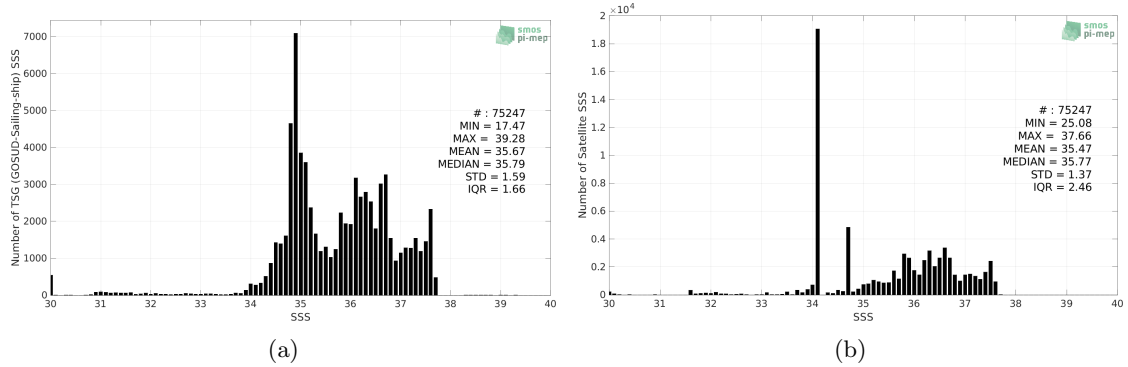
Figure 2: Histograms of SSS from TSG (GOSUD-Sailing-ship) (a) and SMAP SSS L4 OI v2 - Monthly (IPRC) (b) considering all match-up pairs per bins of 0.1 over the Amazon and Orinoco river plumes Pi-MEP region and for the full satellite product period.
