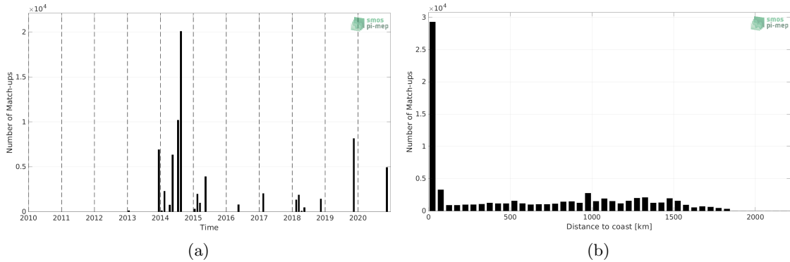
Figure 1: Number of match-ups between TSG (GOSUD-Sailing-ship) and SMAP SSS L4 OI v2 - Monthly (IPRC) SSS as a function of time (a) and as function of the distance to coast (b) over the Amazon and Orinoco river plumes Pi-MEP region and for the full satellite product period.
