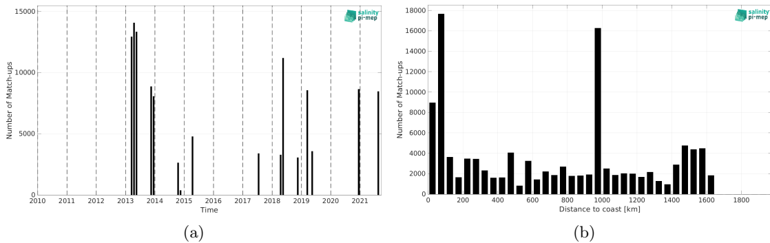
Figure 1: Number of match-ups between TSG (CSIC-UTM) and SMAP SSS L4 OI v2 - Monthly (IPRC) SSS as a function of time (a) and as function of the distance to coast (b) over the Amazon and Orinoco river plumes Pi-MEP region and for the full satellite product period.
