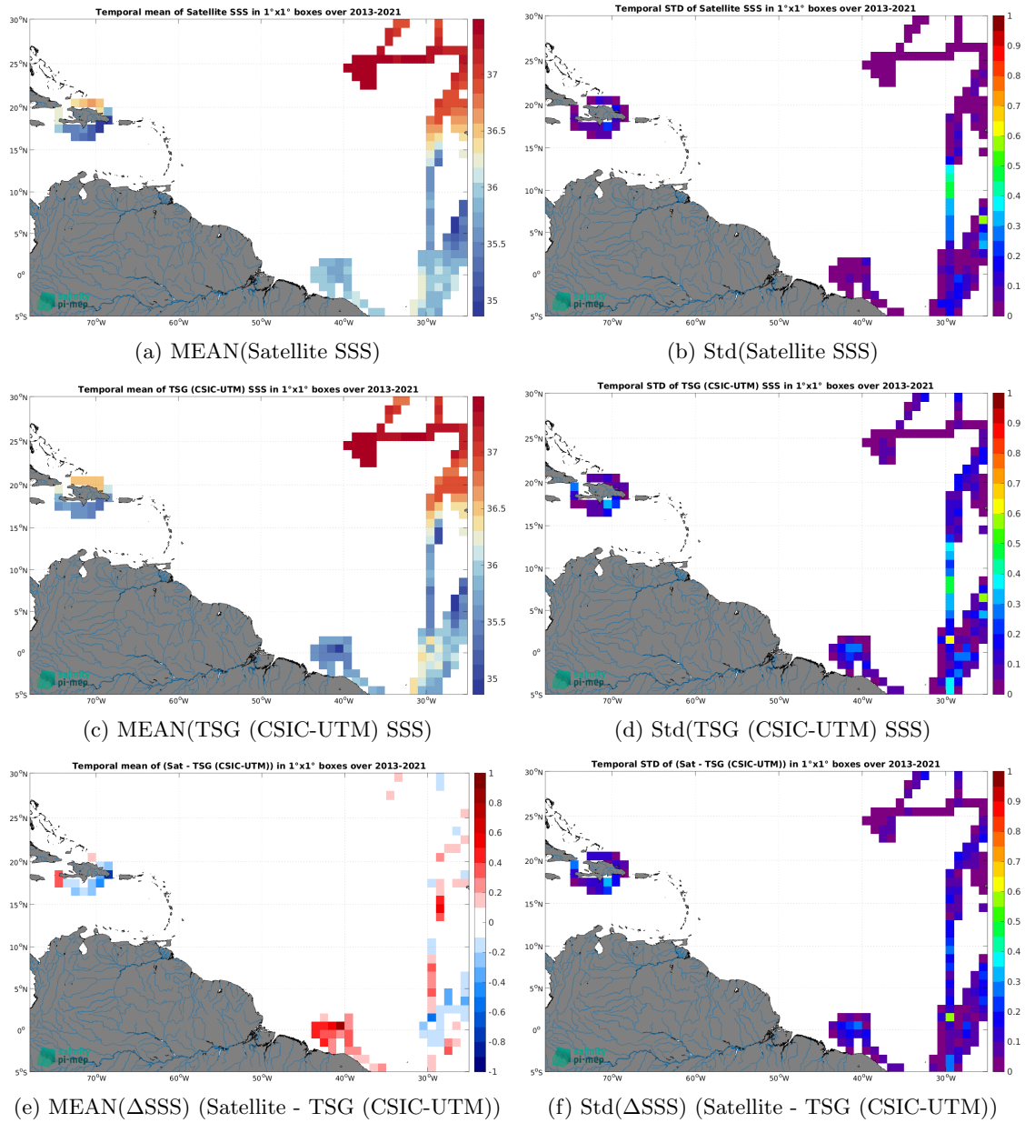
Figure 6: Temporal mean (left) and Std (right) of SSS from SMAP SSS L4 OI v2 - Monthly (IPRC) (top), TSG (CSIC-UTM) (middle), and of \Delta SSS (Satellite - TSG (CSIC-UTM)). Only match-up pairs are used to generate these maps.
