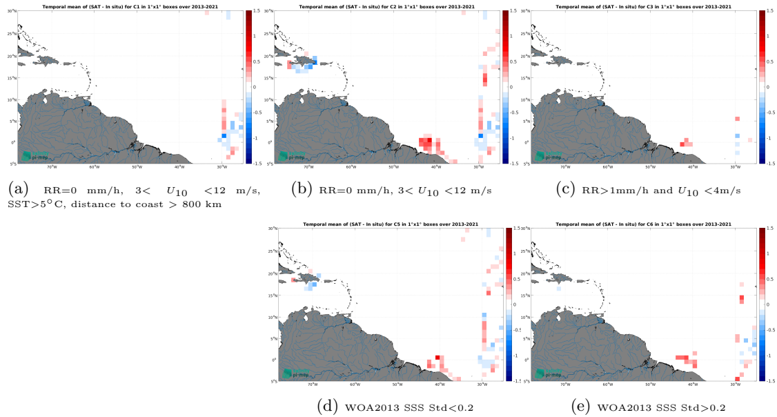
Figure 12: Temporal mean gridded over spatial boxes of size 1^\circ \times 1^\circ of \Delta SSS (SMAP SSS L4 OI v2 - Monthly (IPRC) - TSG (CSIC-UTM)) for 5 different subdatasets corresponding to:RR=0 mm/h, 3 < U_{10} < 12 m/s, SST > 5^\circ\text{C} , distance to coast > 800 km (a), RR=0 mm/h, 3 < U_{10} < 12 m/s (b), RR > 1 mm/h and U_{10} < 4 m/s (c), WOA2013 SSS Std < 0.2 (d), WOA2013 SSS Std > 0.2 (e).
