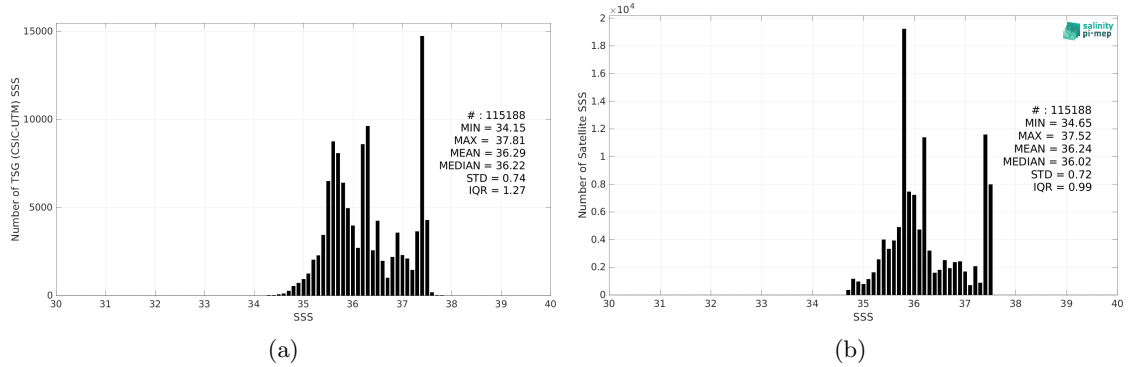
Figure 2: Histograms of SSS from TSG (CSIC-UTM) (a) and SMAP SSS L4 OI v2 - Monthly (IPRC) (b) considering all match-up pairs per bins of 0.1 over the Amazon and Orinoco river plumes Pi-MEP region and for the full satellite product period.
