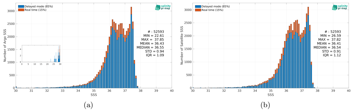
Figure 2: Histograms of SSS from Argo (a) and SMAP SSS L4 OI v2 - Monthly (IPRC) (b) considering all match-up pairs per bins of 0.1 over the Amazon and Orinoco river plumes Pi-MEP region and for the full satellite product period.
