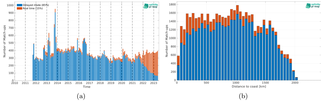
Figure 1: Number of match-ups between Argo and SMAP SSS L4 OI v2 - Monthly (IPRC) SSS as a function of time (a) and as function of the distance to coast (b) over the Amazon and Orinoco river plumes Pi-MEP region and for the full satellite product period.
