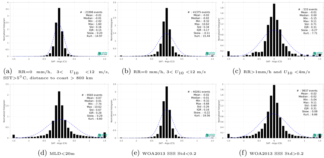
Figure 13: Normalized histogram of \Delta\text{SSS} (SMAP SSS L4 OI v2 - Monthly (IPRC) - Argo) for 6 different subdatasets corresponding to: RR=0 mm/h, 3 < U_{10} < 12 m/s, SST>5°C, distance to coast > 800 km (a), RR=0 mm/h, 3 < U_{10} < 12 m/s (b), RR>1mm/h and U_{10} < 4 m/s (c), MLD<20m (d), WOA2013 SSS Std<0.2 (e), WOA2013 SSS Std>0.2 (f).
