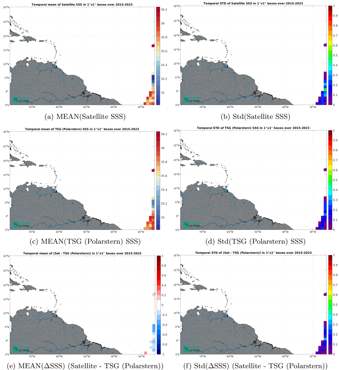
Figure 7: Temporal mean (left) and Std (right) of SSS from SMAP SSS L3 v6 - 8-Day running (RSS) (top), TSG (Polarstern) (middle), and of \Delta SSS (Satellite - TSG (Polarstern)). Only match-up pairs are used to generate these maps.
