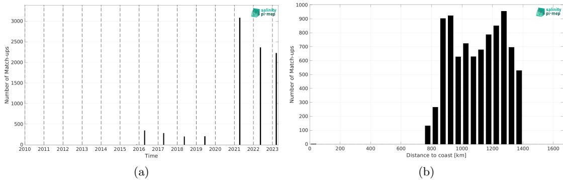
Figure 2: Number of match-ups between TSG (Polarstern) and SMAP SSS L3 v6 - 8-Day running (RSS) SSS as a function of time (a) and as function of the distance to coast (b) over the Amazon and Orinoco river plumes Pi-MEP region and for the full satellite product period.
