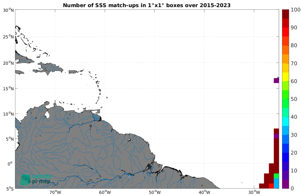
Figure 5: Number of SSS match-ups between TSG (Polarstern) SSS and the SMAP SSS L3 v6 - 8-Day running (RSS) SSS product for the Amazon and Orinoco river plumes Pi-MEP region over 1^\circ \times 1^\circ boxes and for the full satellite product period.
