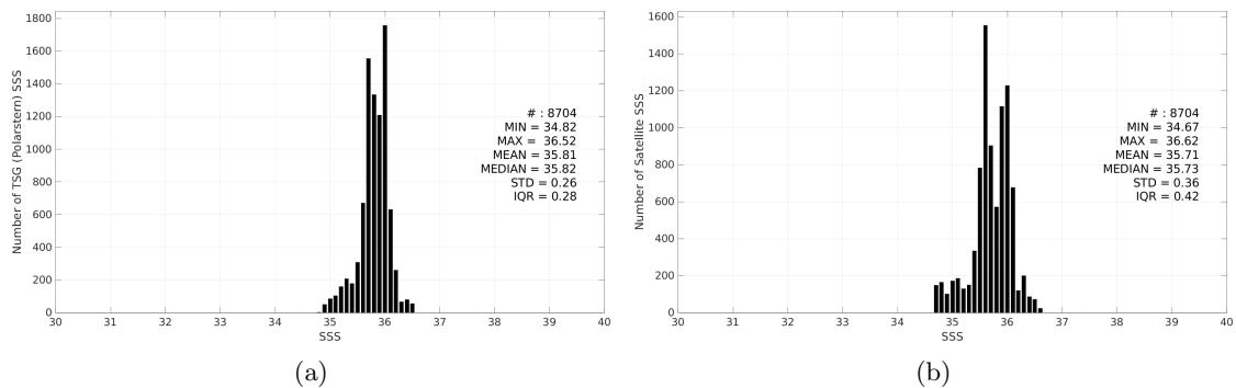
Figure 3: Histograms of SSS from TSG (Polarstern) (a) and SMAP SSS L3 v6 - 8-Day running (RSS) (b) considering all match-up pairs per bins of 0.1 over the Amazon and Orinoco river plumes Pi-MEP region and for the full satellite product period.
