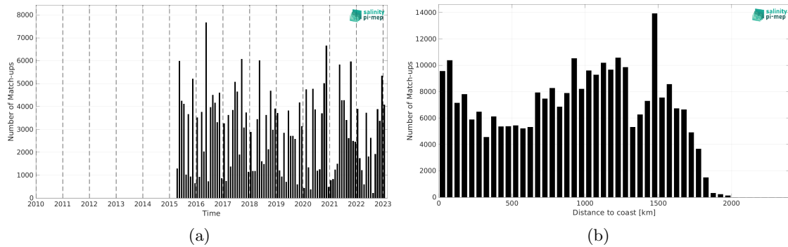
Figure 2: Number of match-ups between TSG (LEGOS-DM) and SMAP SSS L3 v6 - 8-Day running (RSS) SSS as a function of time (a) and as function of the distance to coast (b) over the Amazon and Orinoco river plumes Pi-MEP region and for the full satellite product period.
