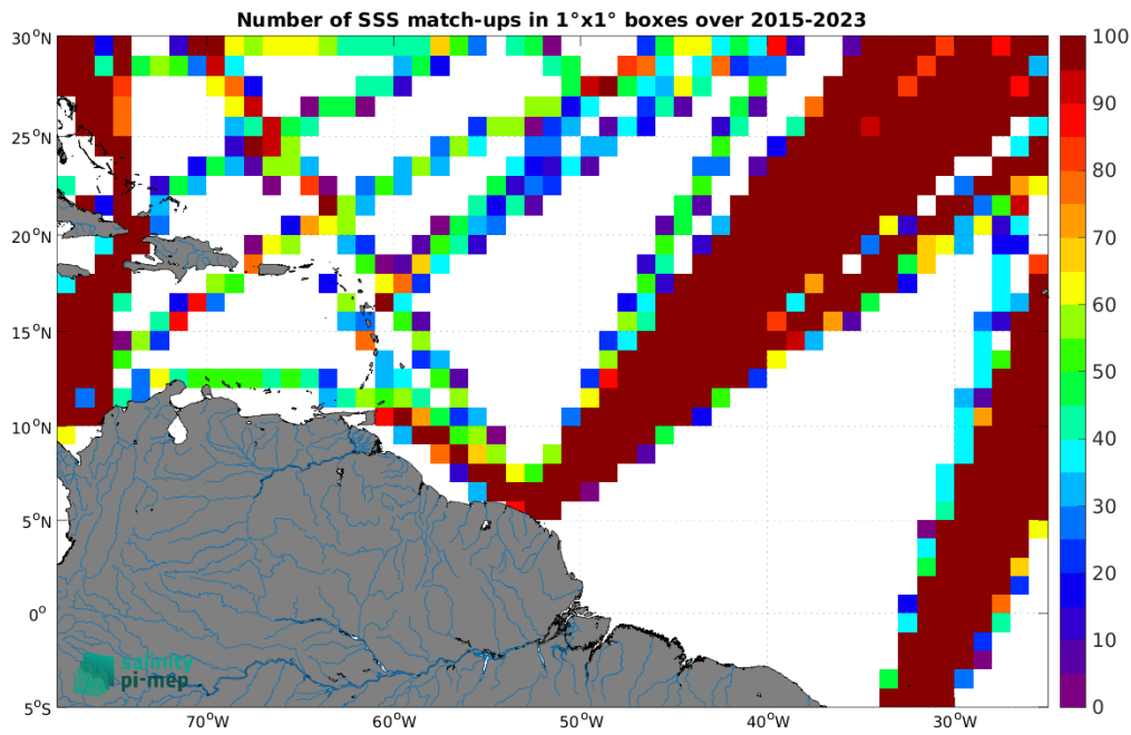
Figure 5: Number of SSS match-ups between TSG (LEGOS-DM) SSS and the SMAP SSS L3 v6 - 8-Day running (RSS) SSS product for the Amazon and Orinoco river plumes Pi-MEP region over 1^\circ \times 1^\circ boxes and for the full satellite product period.
