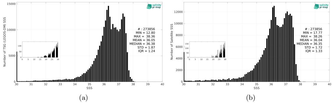
Figure 3: Histograms of SSS from TSG (LEGOS-DM) (a) and SMAP SSS L3 v6 - 8-Day running (RSS) (b) considering all match-up pairs per bins of 0.1 over the Amazon and Orinoco river plumes Pi-MEP region and for the full satellite product period.
