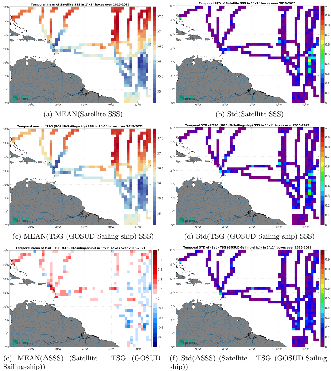
Figure 7: Temporal mean (left) and Std (right) of SSS from SMAP SSS L3 v6 - 8-Day running (RSS) (top), TSG (GOSUD-Sailing-ship) (middle), and of \Delta SSS (Satellite - TSG (GOSUD-Sailing-ship)). Only match-up pairs are used to generate these maps.
