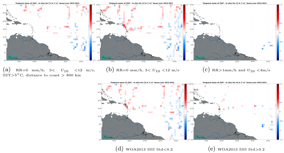
Figure 14: Temporal mean gridded over spatial boxes of size 1^\circ \times 1^\circ of \Delta SSS (SMAP SSS L3 v6 - 8-Day running (RSS) - TSG (GOSUD-Sailing-ship)) for 5 different subdatasets corresponding to:RR=0 mm/h, 3 < U_{10} < 12 m/s, SST>5°C, distance to coast > 800 km (a), RR=0 mm/h, 3 < U_{10} < 12 m/s (b), RR>1mm/h and U_{10} < 4 m/s (c), WOA2013 SSS Std<0.2 (d), WOA2013 SSS Std>0.2 (e).
