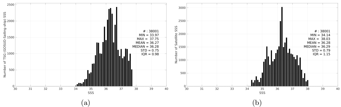
Figure 3: Histograms of SSS from TSG (GOSUD-Sailing-ship) (a) and SMAP SSS L3 v6 - 8-Day running (RSS) (b) considering all match-up pairs per bins of 0.1 over the Amazon and Orinoco river plumes Pi-MEP region and for the full satellite product period.
