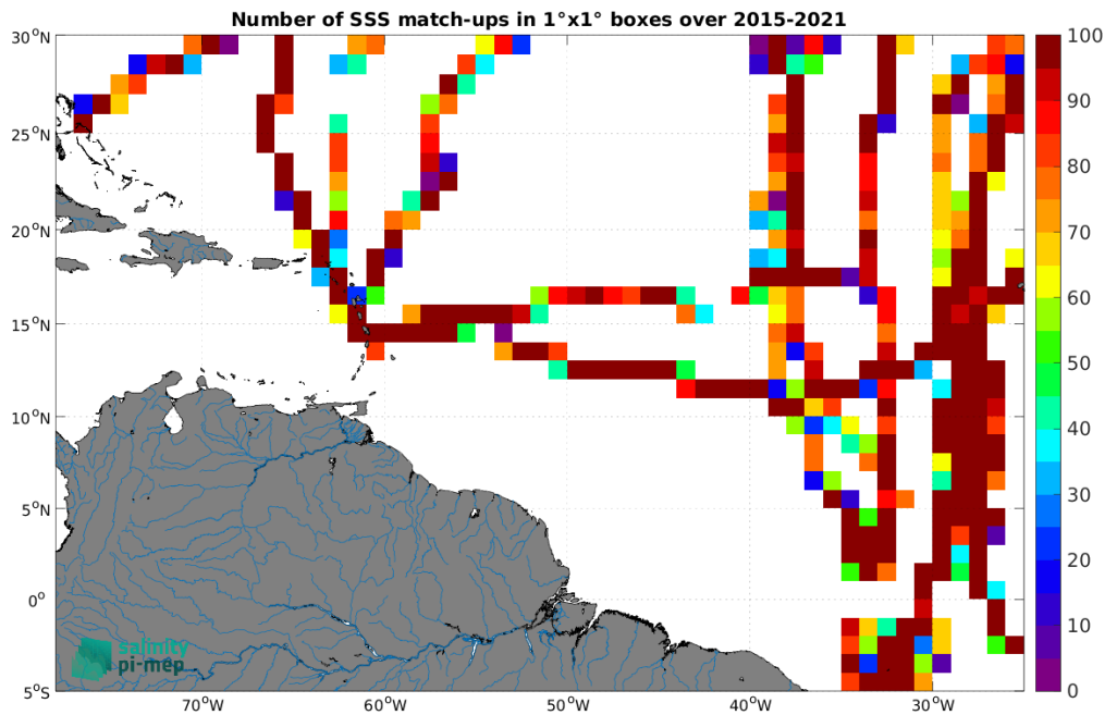
Figure 5: Number of SSS match-ups between TSG (GOSUD-Sailing-ship) SSS and the SMAP SSS L3 v6 - 8-Day running (RSS) SSS product for the Amazon and Orinoco river plumes Pi-MEP region over 1^{\circ} \times 1^{\circ} boxes and for the full satellite product period.
