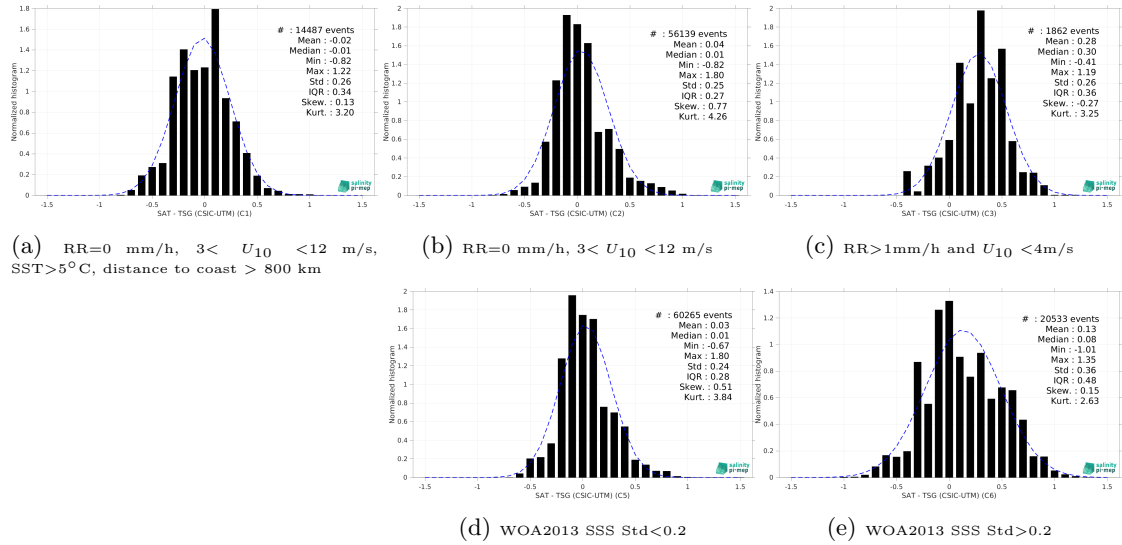
Figure 15: Normalized histogram of \Delta\text{SSS} (SMAP SSS L3 v6 - 8-Day running (RSS) - TSG (CSIC-UTM)) for 5 different subdatasets corresponding to: RR=0 mm/h, 3 < U_{10} < 12 m/s, SST>5°C, distance to coast > 800 km (a), RR=0 mm/h, 3 < U_{10} < 12 m/s (b), RR>1mm/h and U_{10} < 4 m/s (c), WOA2013 SSS Std<0.2 (d), WOA2013 SSS Std>0.2 (e).
